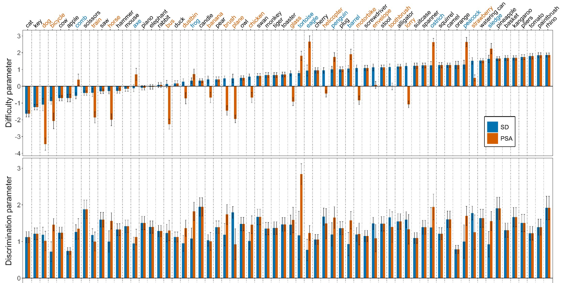
Figure 2. Difficulty and discrimination parameters of each item for the Final IRT models. Items are sorted by increasing difficulty based on the SD item parameters. Error bars indicate Standard Error of the estimated item parameter. Coloured words indicate that the DIF was significant. Blue-coloured words indicate that the item is systematically easier for SD than for PSA patients, orange-coloured words vice versa.
