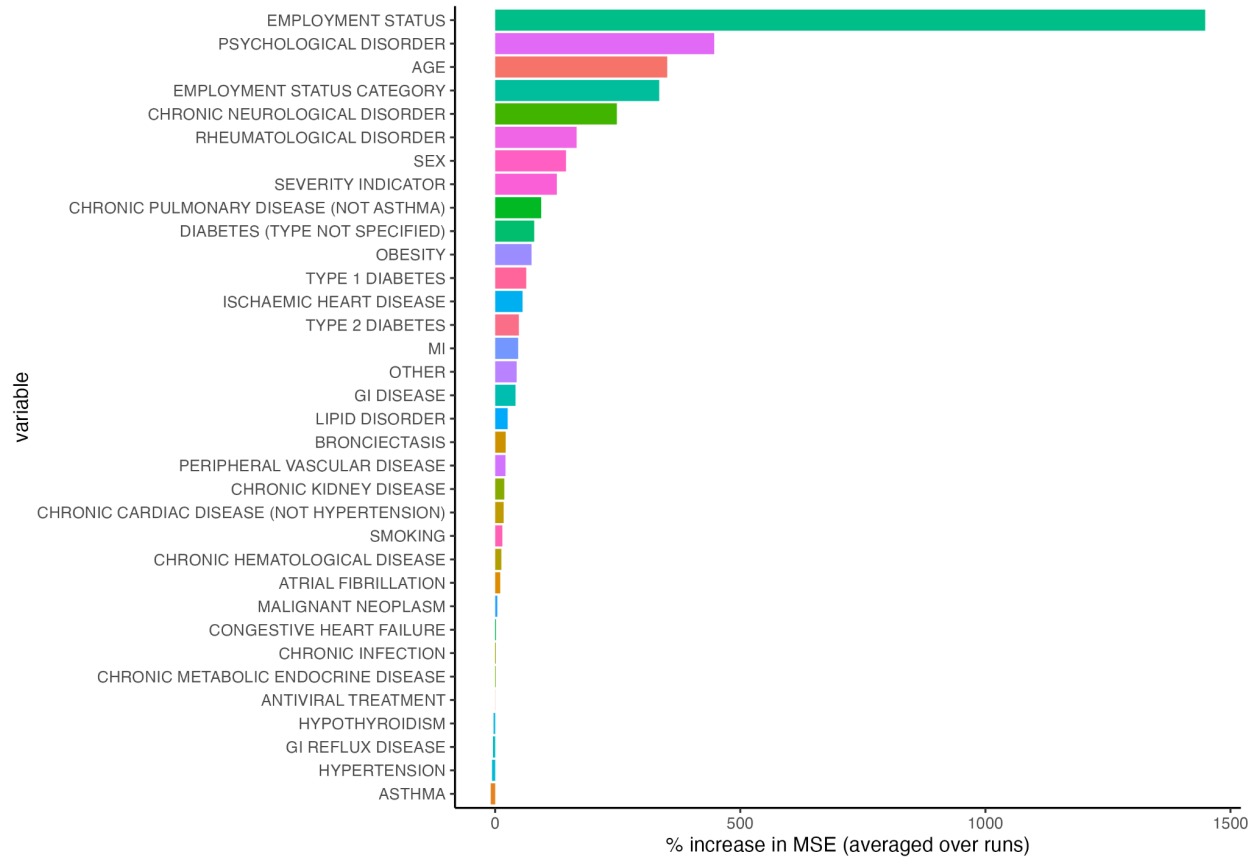
Supplementary Figure S13a. Estimated variable importance measures, i.e. % increase in mean squared error or MSE, from individual random forest implementation (RF #1) for the UK (sex-based population correction sensitivity analysis).
