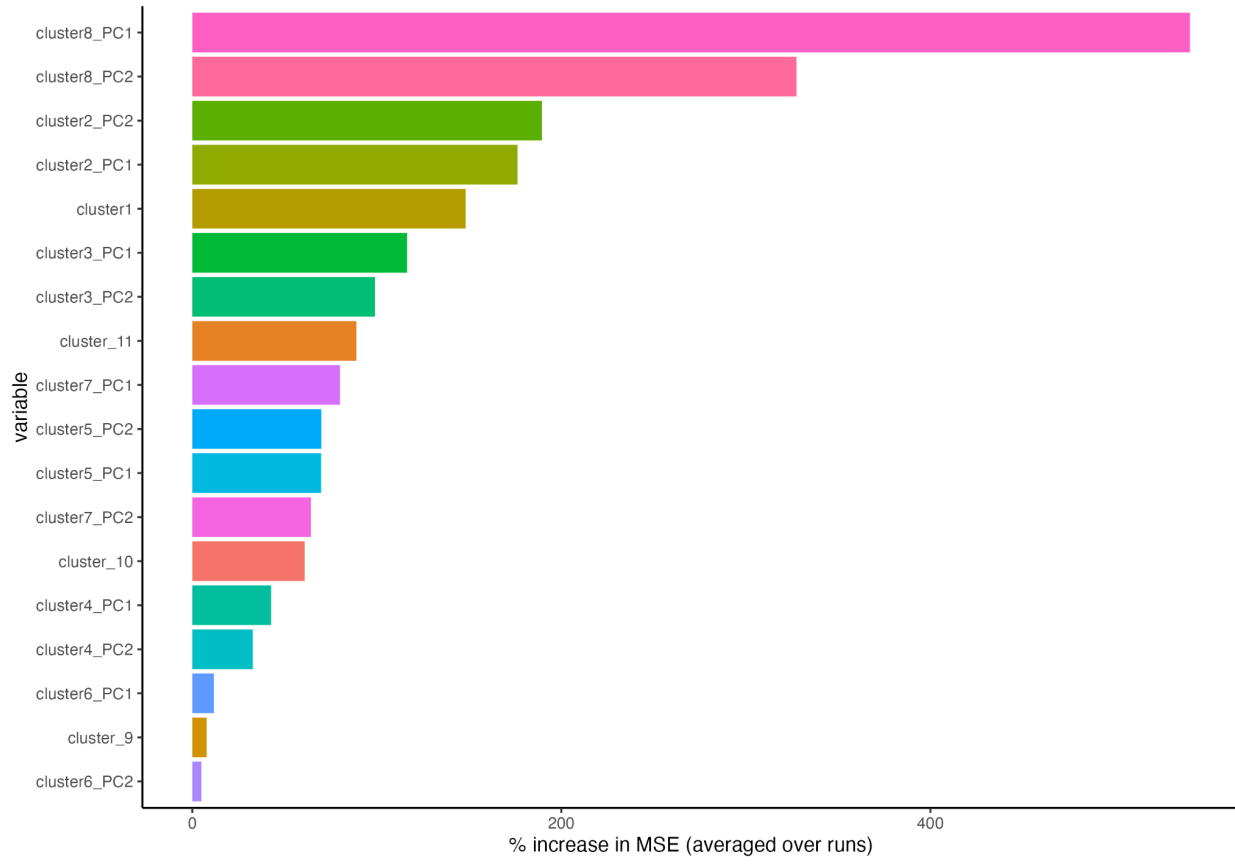
Supplementary Figure S12c. Estimated variable importance measures, i.e. % increase in mean squared error or MSE, from pre-grouped random forest implementation (RF #2) for Norway. Rows indicate cluster names (a full list of variables belonging to each cluster can be found in Supplementary Table S3) and corresponding principal components, if the cluster consists of multiple variables. PC1 denotes principal component 1 and PC2 denotes principal component 2 (sex-based population correction sensitivity analysis).
