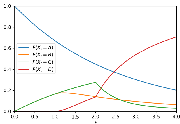
Figure 3: The resulting process X_t from the model illustrated in Figure 2
