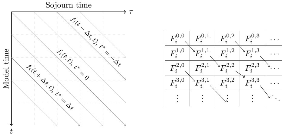
Figure 1: Characteristics of constant t^* = t - \tau for f_i(t, \tau) (left) and the corresponding elements F_i^{m,n} with constant m - n for the numerical scheme (right).
