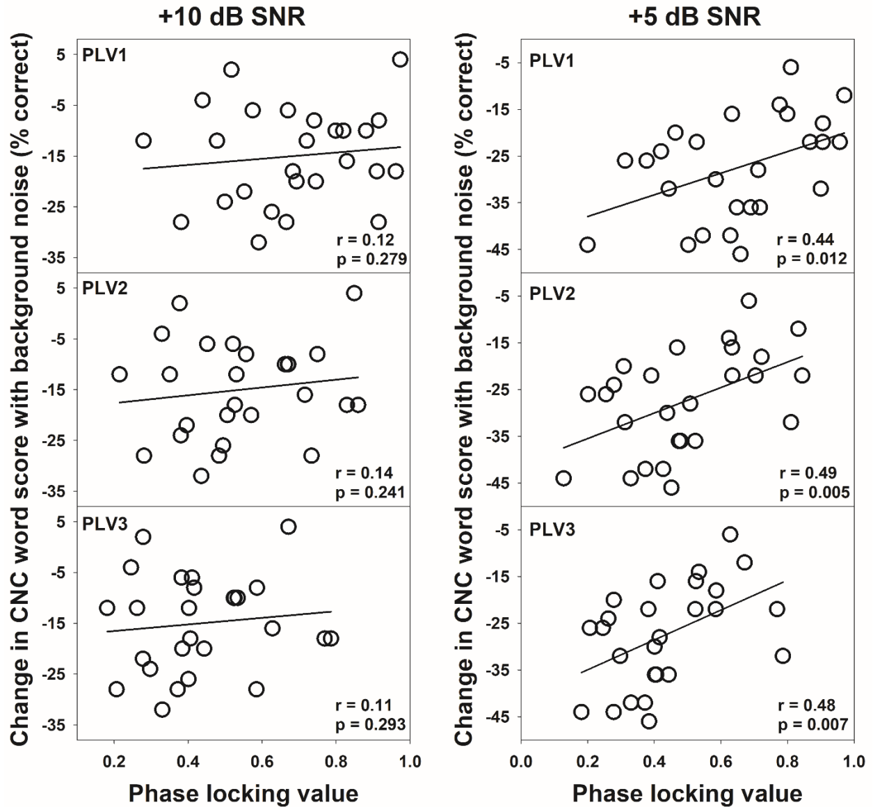
Figure C1. The change in Consonant-Nucleus-Consonant (CNC) word scores with the addition of background noise as a function of the averaged phase-locking value (PLV) across electrode locations. PLVs calculated using different sets of parameters are indicated in different rows (PLV1, PLVs calculated using Parameter set I; PLV2, PLVs calculated using Parameter set II; PLV3, PLVs calculated using Parameter set III). Each column indicates results measured in each testing condition. The best fit line across all
