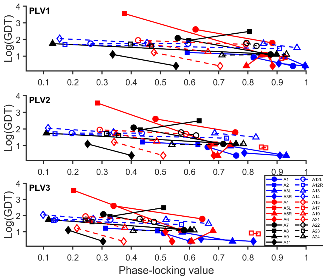
Figure A 1. Phase-locking values calculated using different sets of parameters (PLV1, PLVs calculated using Parameter set I; PLV2, PLVs calculated using Parameter set II; PLV3, PLVs calculated using Parameter set III) and psychophysical gap detection thresholds measured at two electrode locations in each of 23 implanted ears of 20 participants. Lines connect the data measured at the two electrode locations tested in the same ear.
