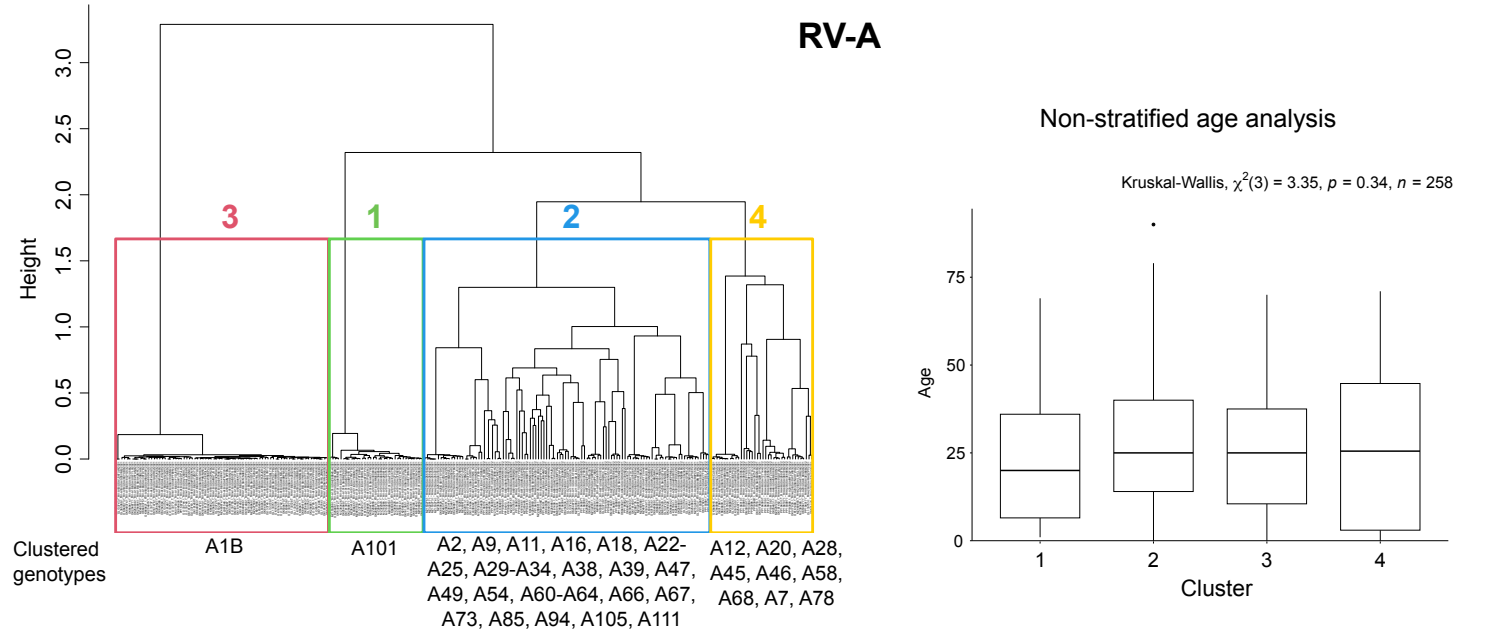
Supplementary Figure 3. Hierarchical cluster analysis of the polyprotein-based pairwise genetic distance matrix. Principal component analysis (PCA) and hierarchical clustering was calculated from the pairwise genetic distance between the polyprotein sequence for each RV species. The number of clusters was defined by within-cluster sum of squares method. Each numbered cluster is highlighted with a colored squared including the detail of the genotypes clustering together. At the right of each dendrogram the analysis of association between age of the individuals and the clusters obtained is shown.
