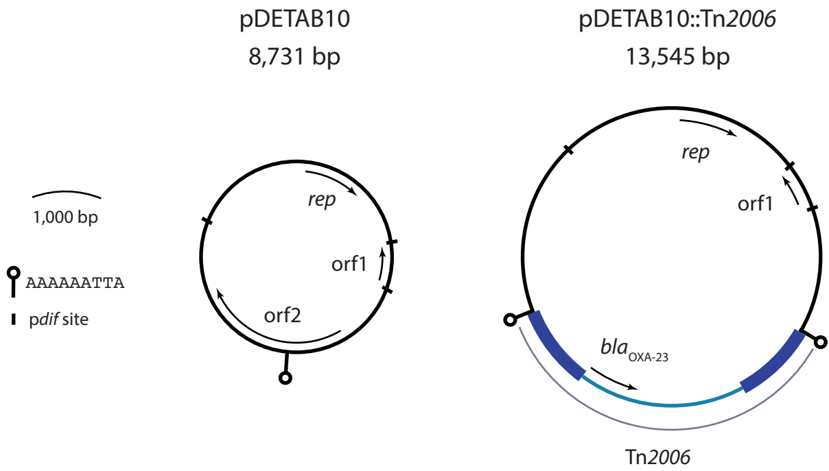
Figure S4: Acquisition of Tn2006 by pDETAB10. Scaled schematic diagrams of the R3-T1 plasmids pDETAB10 and pDETAB10::Tn2006. The plasmid backbone is shown as a black line, the insertion sequence ISAb a1 as navy boxes, and the Tn2006 passenger segment as a light blue line. Open reading frames are shown as labelled arrows. The locations of target site duplications and pdif sites are indicated as shown in the key to the left of the figure.
