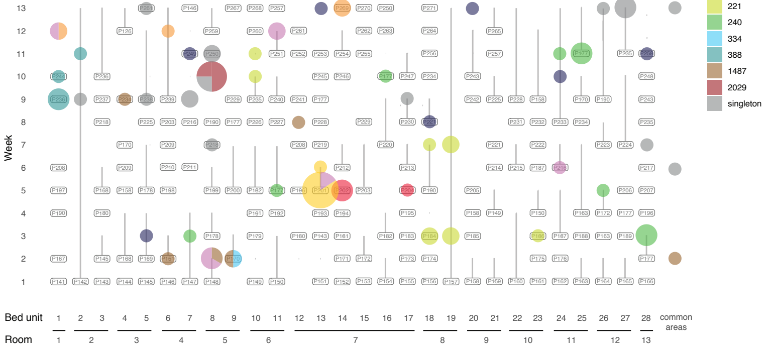
Figure S3: Spatiotemporal distribution of carbapenem-sensitive Acinetobacter baumannii (CSAB) in A) patient and B) environmental samples. Coloured circles correspond to the sequence type (ST) and number of isolates collected from each bed unit or patient at each time point, as outlined in the key to the right of the figure.
