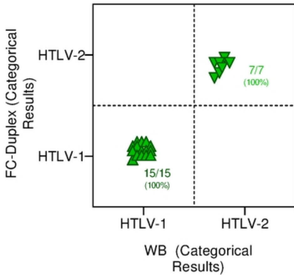
b) Western Blot vs FC-Duplex IgG1 - (2023)
