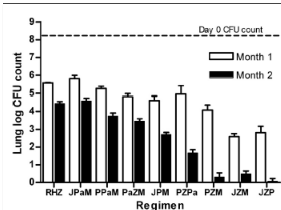
Figure 1 Mean lung log 10 CFU counts (±SD) after 1 and 2 months of treatment
