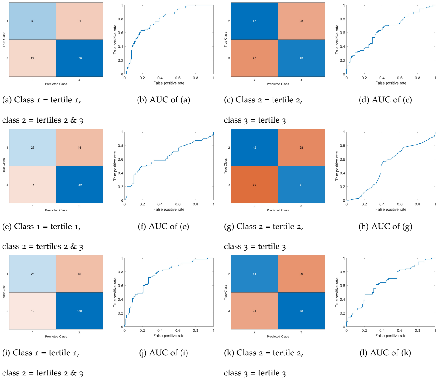
Figure 2: Confusion matrices and AUCs obtained from ten-fold cross-validated GAM-based binary classification of CAC tertiles using patient characteristics (a)-(d), tooth-loss (e)-(h), and combined patient characteristics and tooth-loss (i)-(l).
