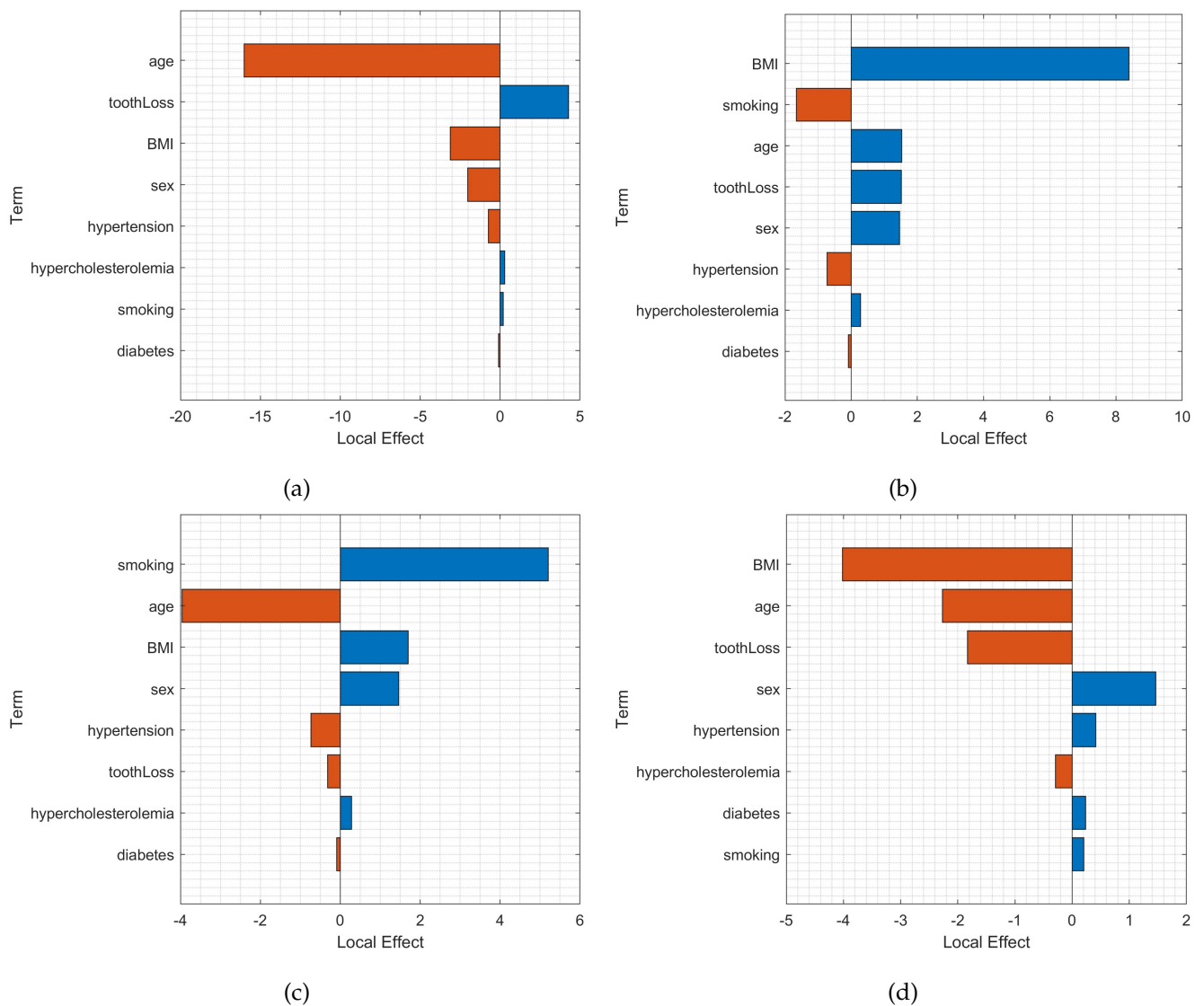
Figure 4: Local effects in: (a) correct classification of tertile 2 for a female patient (age = 36 years, smoking = never, diabetes = no, hypercholesterolemia = no, hypertension = no, BMI = 30.3, and tooth loss = 12); (b) correct classification of tertile 3 for a male patient (age = 66 years, smoking = never, diabetes = no, hypercholesterolemia = no, hypertension = no, BMI = 22.64, and tooth loss = 32); (c) misclassifying tertile 2 as tertile 3 for a male patient (age = 73 years, smoking = never, diabetes = yes, hypercholesterolemia = yes, hypertension = yes, BMI = 25.25, and tooth loss = 7); and (d) misclassifying tertile 3 as tertile 2 for a male patient (age = 56 years, smoking = never, diabetes = no, hypercholesterolemia = no, hypertension = no, BMI = 23.99, and tooth loss = 16).
