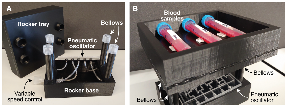
Figure 3: (A) This 3D-printed laboratory rocker/shaker is powered by our pneumatic oscillator. Four plastic bellows are connected to the pneumatic oscillator's outputs by tubing. (B) A tray sits on top of the bellows and holds samples for agitation.
