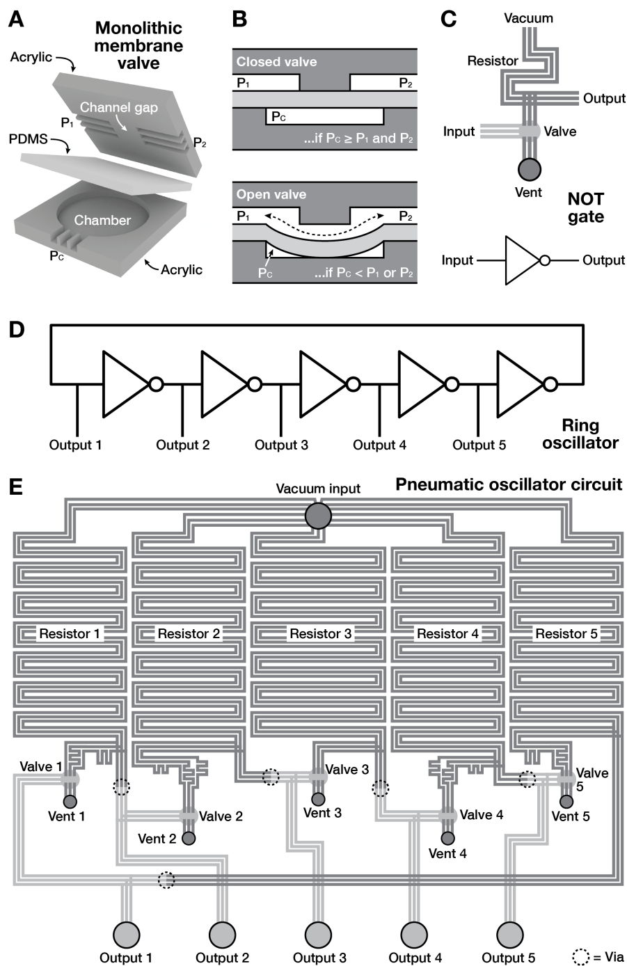
Figure 1: Exploded (A) and cross-section (B) views of a single high-flow monolithic membrane valve. Combining a valve with a vent hole and a long pneumatic resistor channel creates a Boolean NOT gate (C) represented by the symbol shown. An odd number of NOT gates arranged in a loop creates a ring oscillator (D). Design of a pneumatic ring oscillator with five outputs (E). When a constant vacuum is applied to the vacuum input, the five outputs automatically and continuously oscillate between vacuum and atmospheric pressure, all at the same frequency but offset in time (out of phase).
