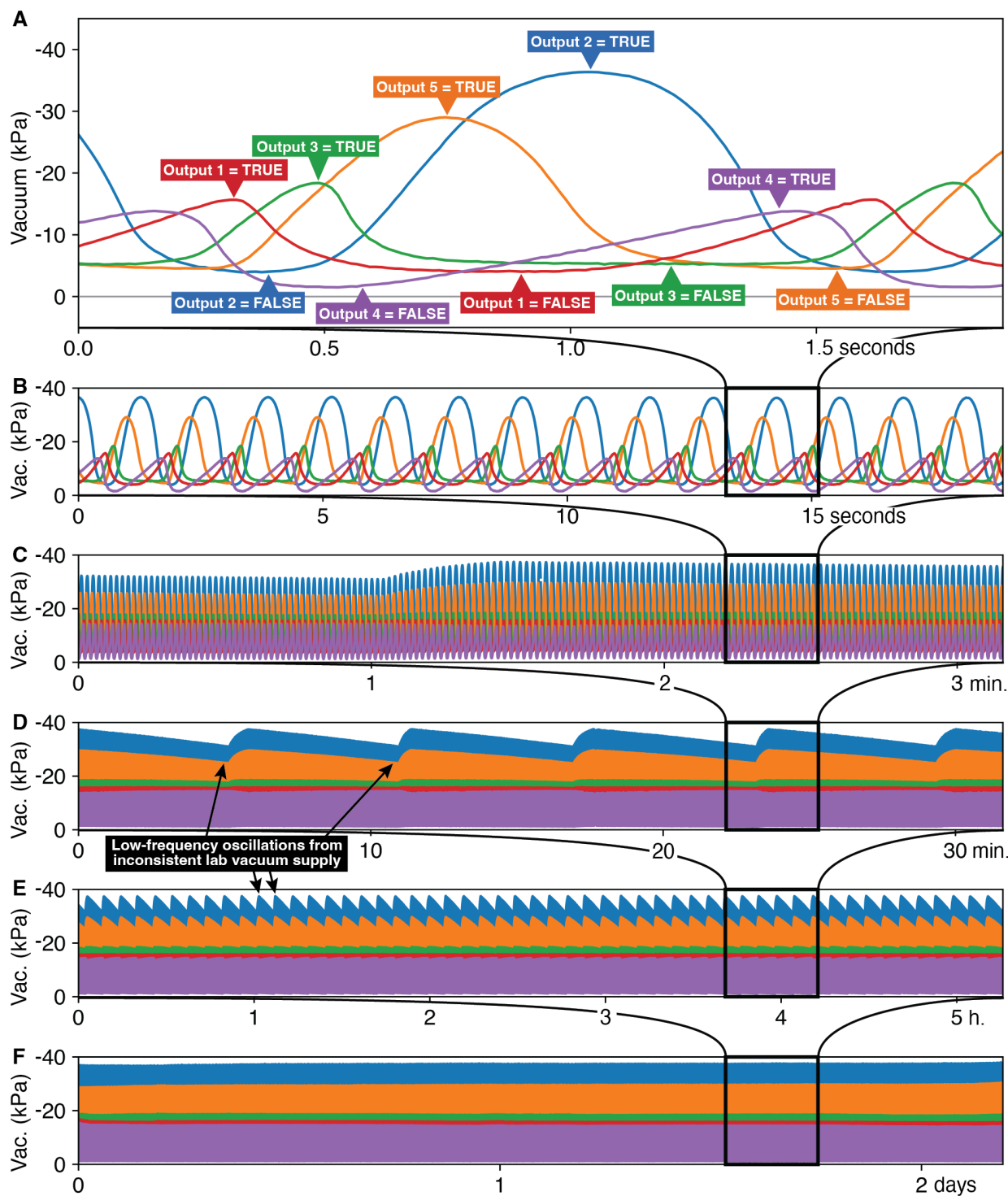
Figure 4: Vacuum pressure measured at each of the five pneumatic oscillator outputs versus time during two days of nonstop operation, zooming out by successive factors of ten to view 1.5 seconds (A), 15 seconds (B), 3 minutes (C), 30 minutes (D), 5 hours (E), and the full 2 days (F). Pressures are relative to atmospheric pressure (0 kPa) and plotted so that higher-magnitude vacuums are higher on the Y-axis.
