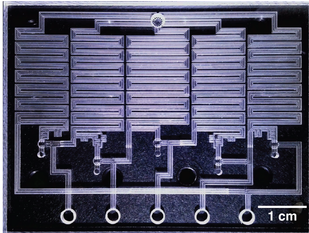
Figure 2: Photograph of a completed high-flow pneumatic oscillator. A single constant vacuum source at the top input powers five outputs at the bottom that automatically oscillate between vacuum and atmospheric pressure.
