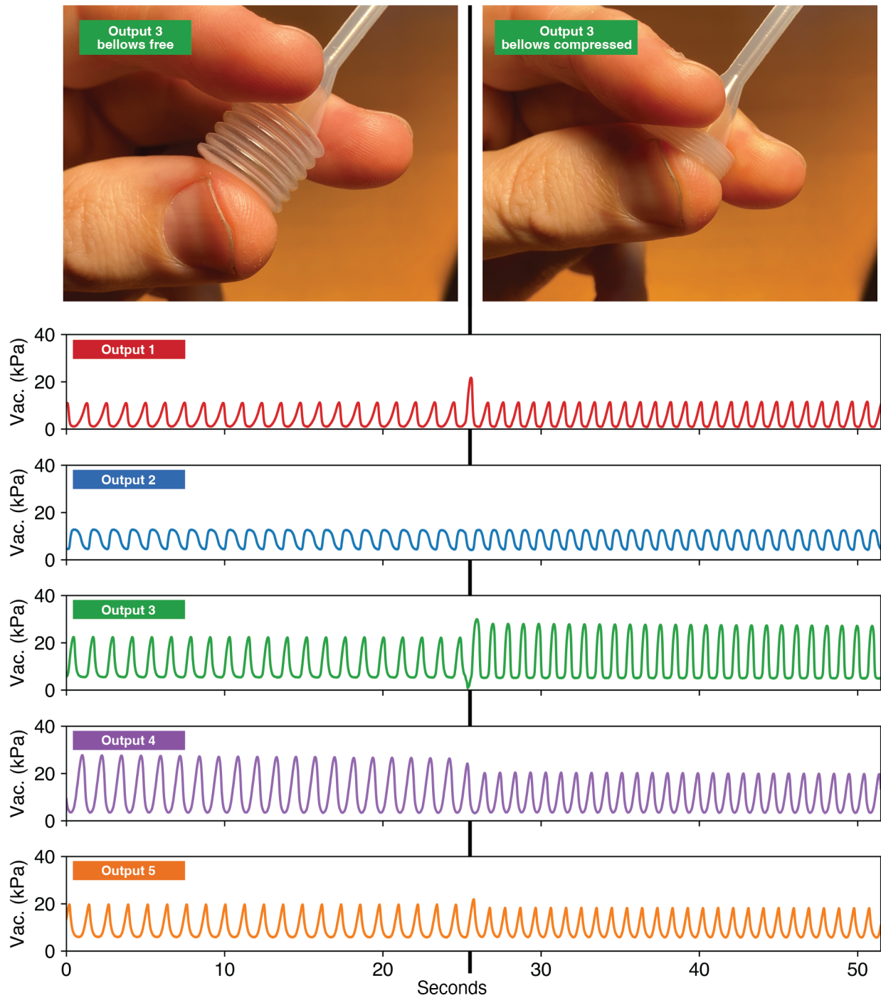
Figure 6: Vacuum pressure measured inside each of the five outputs of the pneumatic oscillator, with the “variable speed control” bellows on output 3 free (0 to 26 seconds) and manually compressed (26 to 50 seconds). Holding the “variable speed control” bellows increases the pneumatic oscillator’s speed by 33%.
