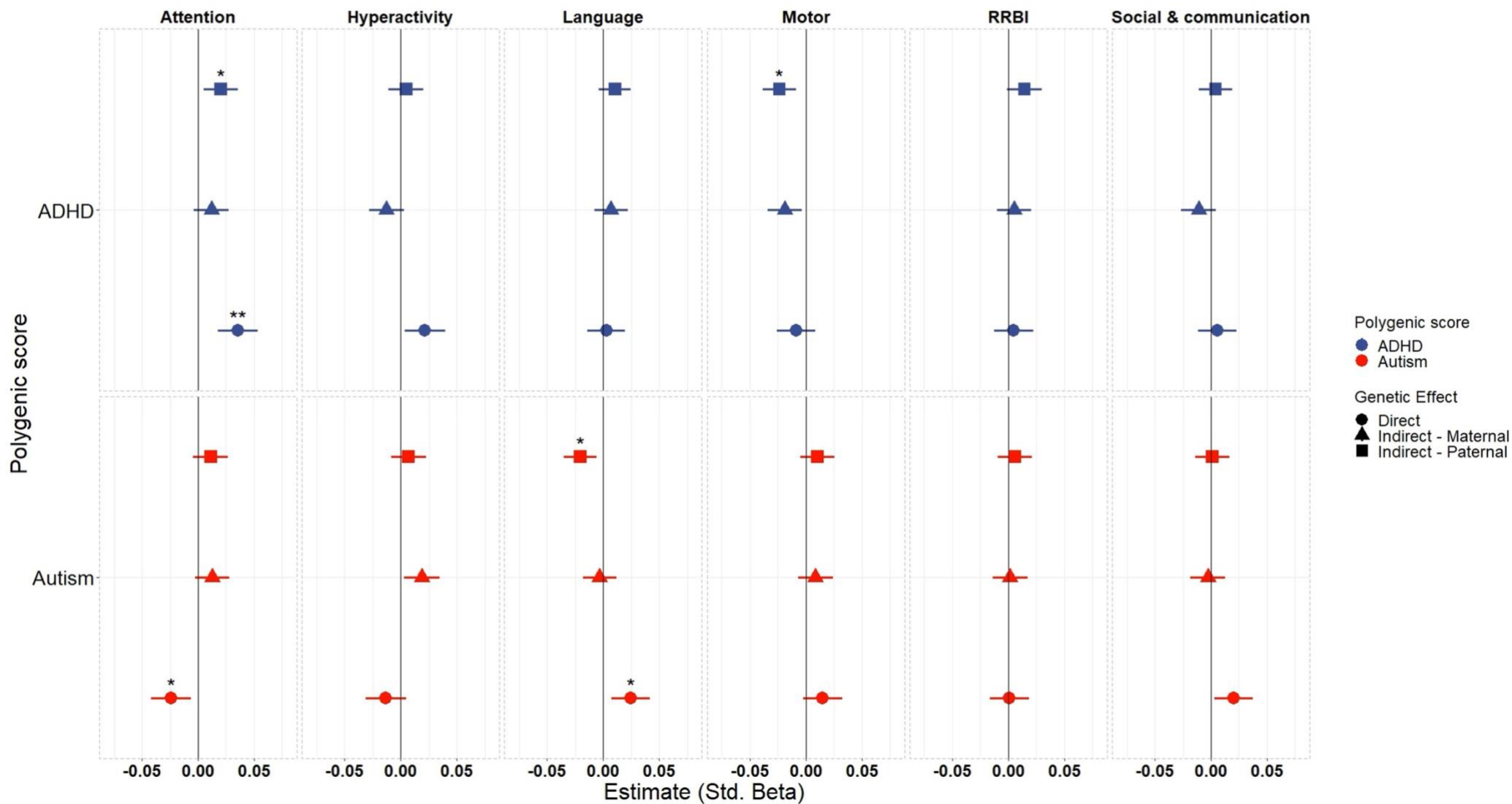
Figure 2: Standardized beta estimates for ADHD and Autism PGS on the six measures of early neurodevelopmental traits. 95% confidence intervals are shown. “*”, “**”, “***” denote adjusted p-values <0.05, <0.01, and <0.001 after multiple testing correction. All results presented are the PGS effect adjusting for the effect of the PGS for the other members of the trio.
