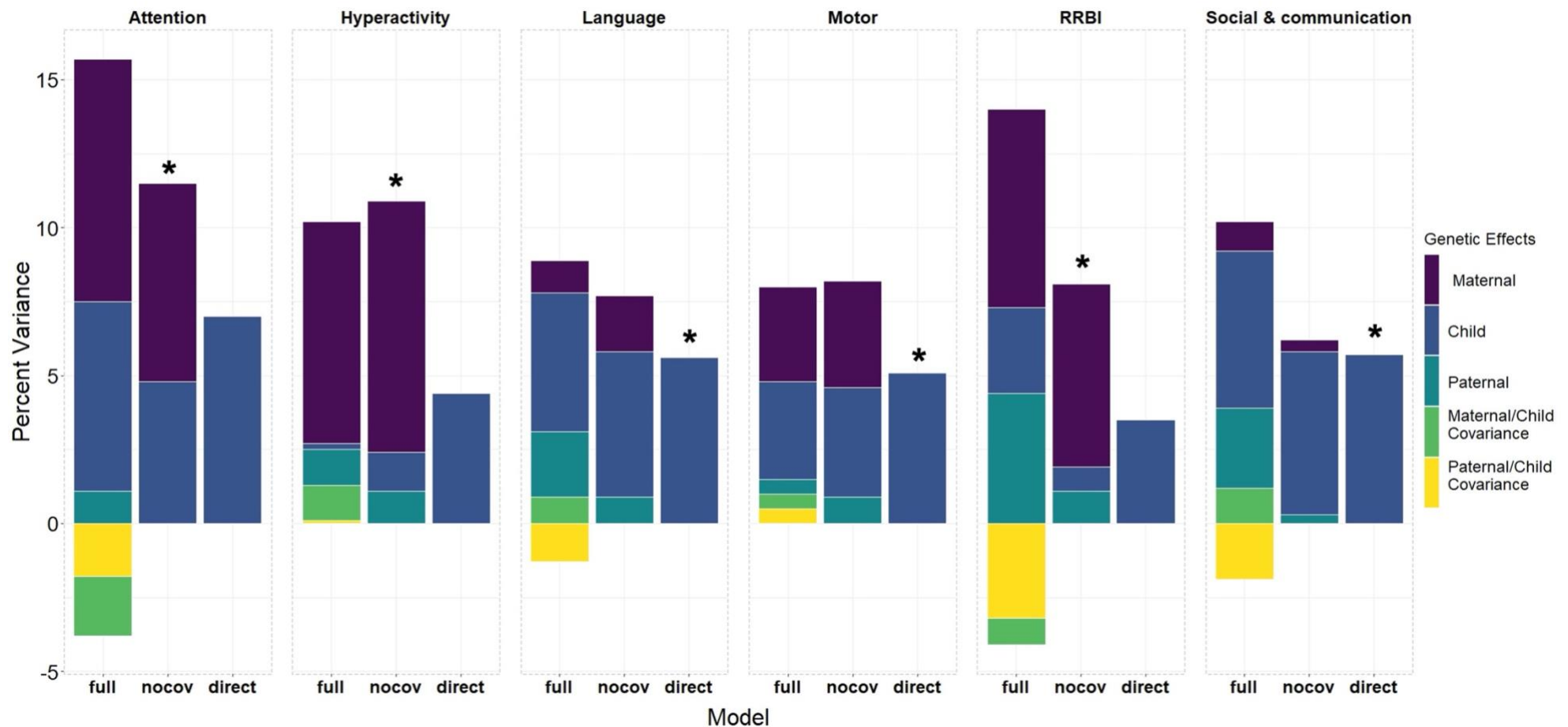
Figure1: Variance component estimates for the full model estimating all parameters, the model not including covariances (nocov), and the direct effects only model. The best fitting model based on AIC is indicated with a “*”. Indirect effects include the variance explained by the genotypes of the mother and father while direct effects are the variance explained by the genotype of the child. In the full models, the covariance between the mother and child’s genetic effects and father and child’s genetic effects is estimated. This represents the extent to which the same genetic variation contributes to maternal/paternal direct and indirect genetic effects. However, when the covariance between direct and indirect effects is negative, the true proportion of variance explained in the outcome by direct and indirect genetic effects is reduced as the effects cancel each other out.
