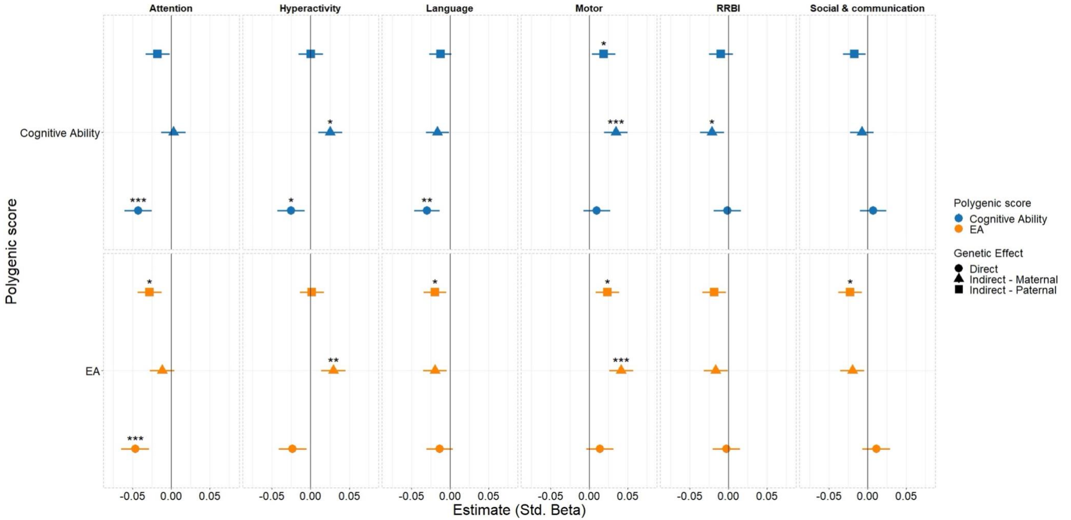
Figure 3: Standardized beta estimates for cognitive ability and educational attainment (EA) PGS on the six measures of early neurodevelopmental traits. 95% confidence intervals are shown. “*”, “**”, “***” denote adjusted p-values <0.05, <0.01, and <0.001 after multiple testing correction. All results presented are the PGS effect adjusting for the effect of the PGS for the other members of the trio.
