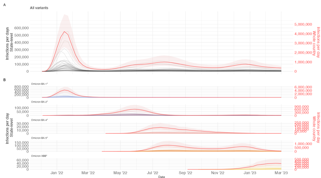
Fig. 1. Time series of daily Omicron variant infections across the entire United States.
