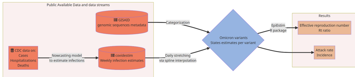
Fig. S1. Flowchart of the process of joining genomic and epidemiological data streams. From the genomic sequences metadata GISAID and infection estimates from covidestim , we produced infection estimates by multiplying the frequencies of each Omicron variant by the infection estimates. Those estimates are then imputed to EpiEstim functions to produce variant-specific effective reproduction numbers, R_t , and state attack rates.
