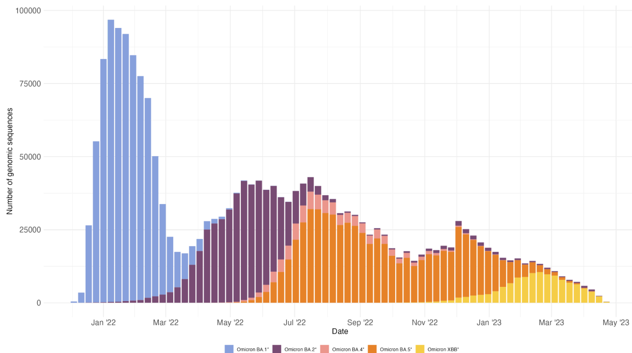
Fig. S2. Number of genomic sequences per variant category per week during the period of December 1st, 2021 to May 1st, 2023, to the whole country. From the GISAID metadata, we calculate the amount of sequences deposited to the database per week, during the analyzed period. Each bar is a week of the period and the filling of the bar is the frequency of each variant during that week. It is possible to see the pattern of succession of variants over the year.
