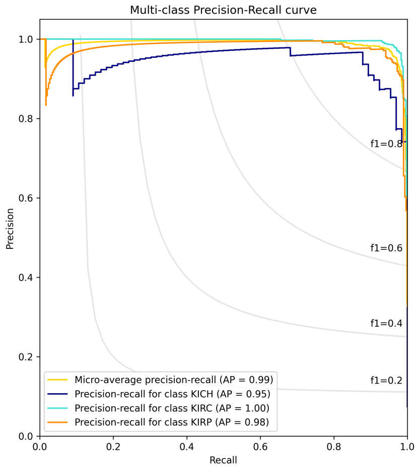
Fig. 6: KIPAN Precision Recall Curve
