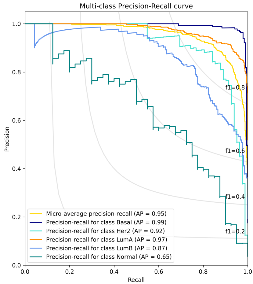
Fig. 5: BRCA Precision Recall Curve
