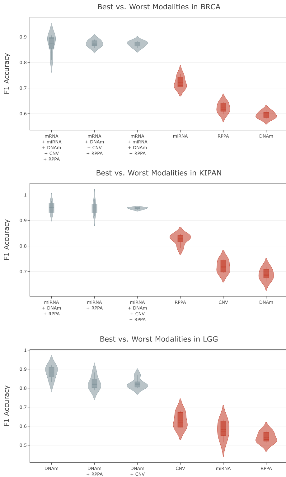
Fig. 2: Best and Worst Performing Modalities in Each Dataset
