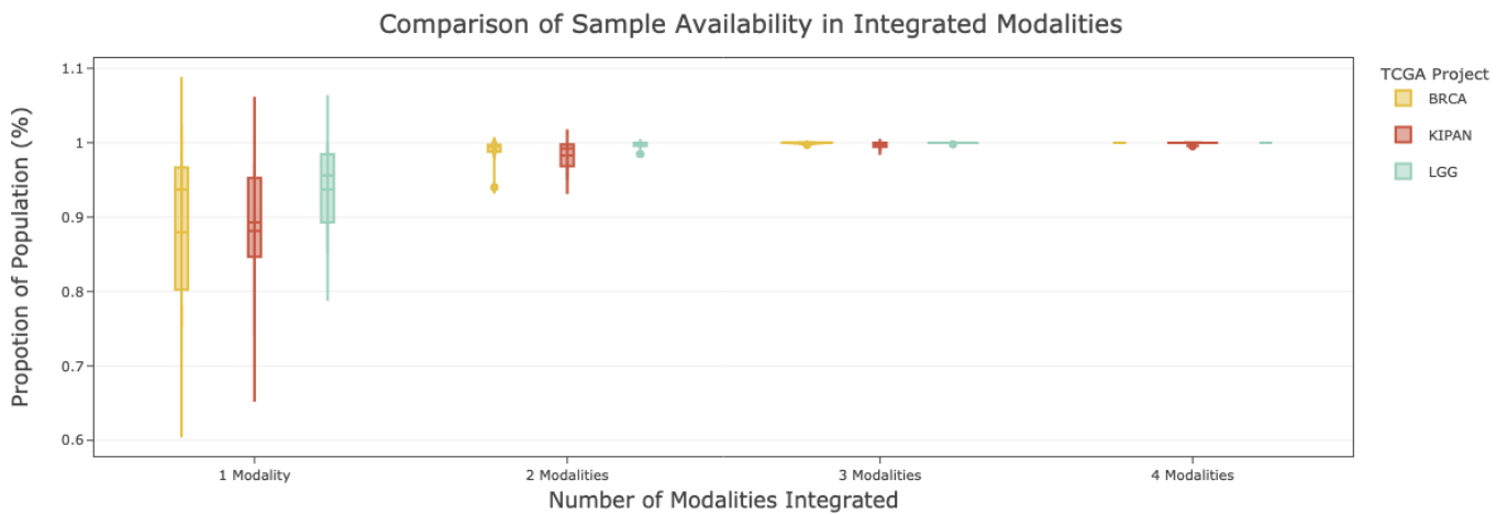
Fig. 4: Percentage of Samples Included when Integrating Modalities
