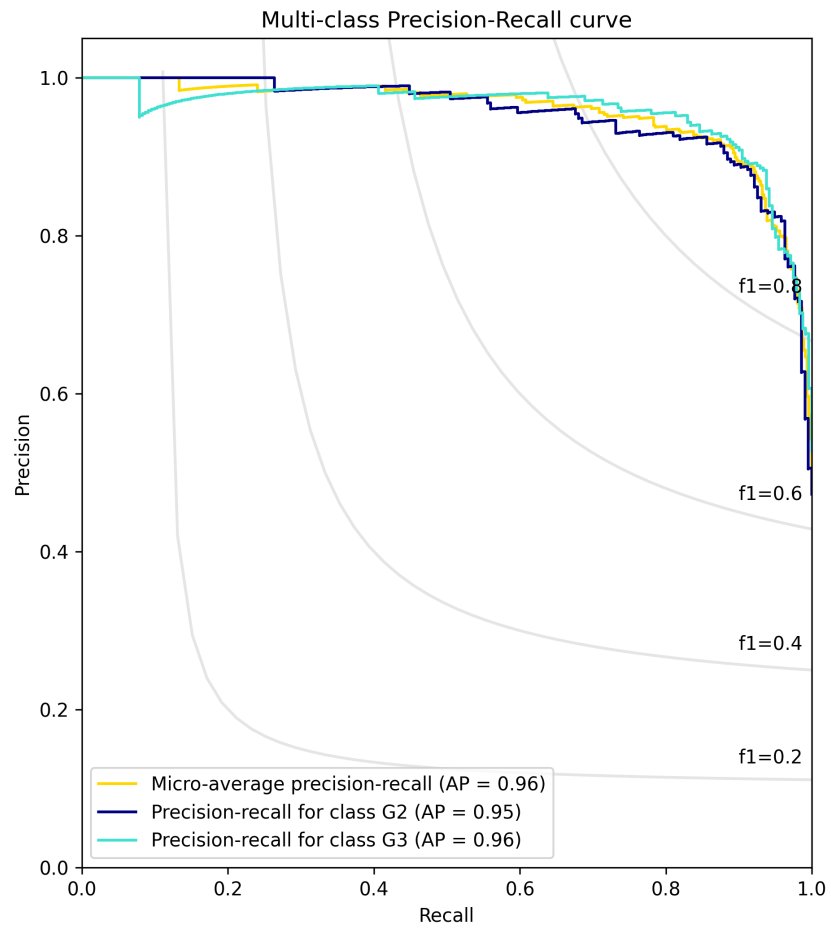
Fig. 7: LGG Precision Recall Curve
