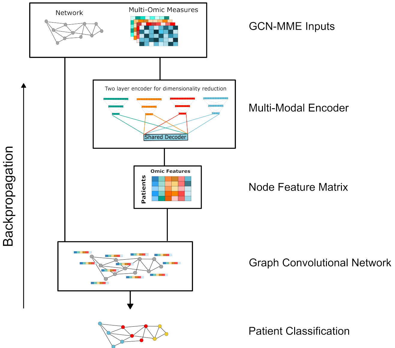
Fig. 1: Graph Convolutional Network - Multi-Modal Encoder Architecture
