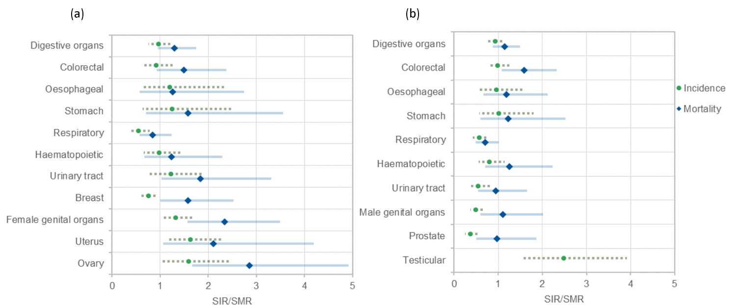
Figure 2. Age- sex- standardised rate ratios of commonest cancer incidence and mortality comparing adults with and without intellectual disabilities for (a) Females and (b) Males.
