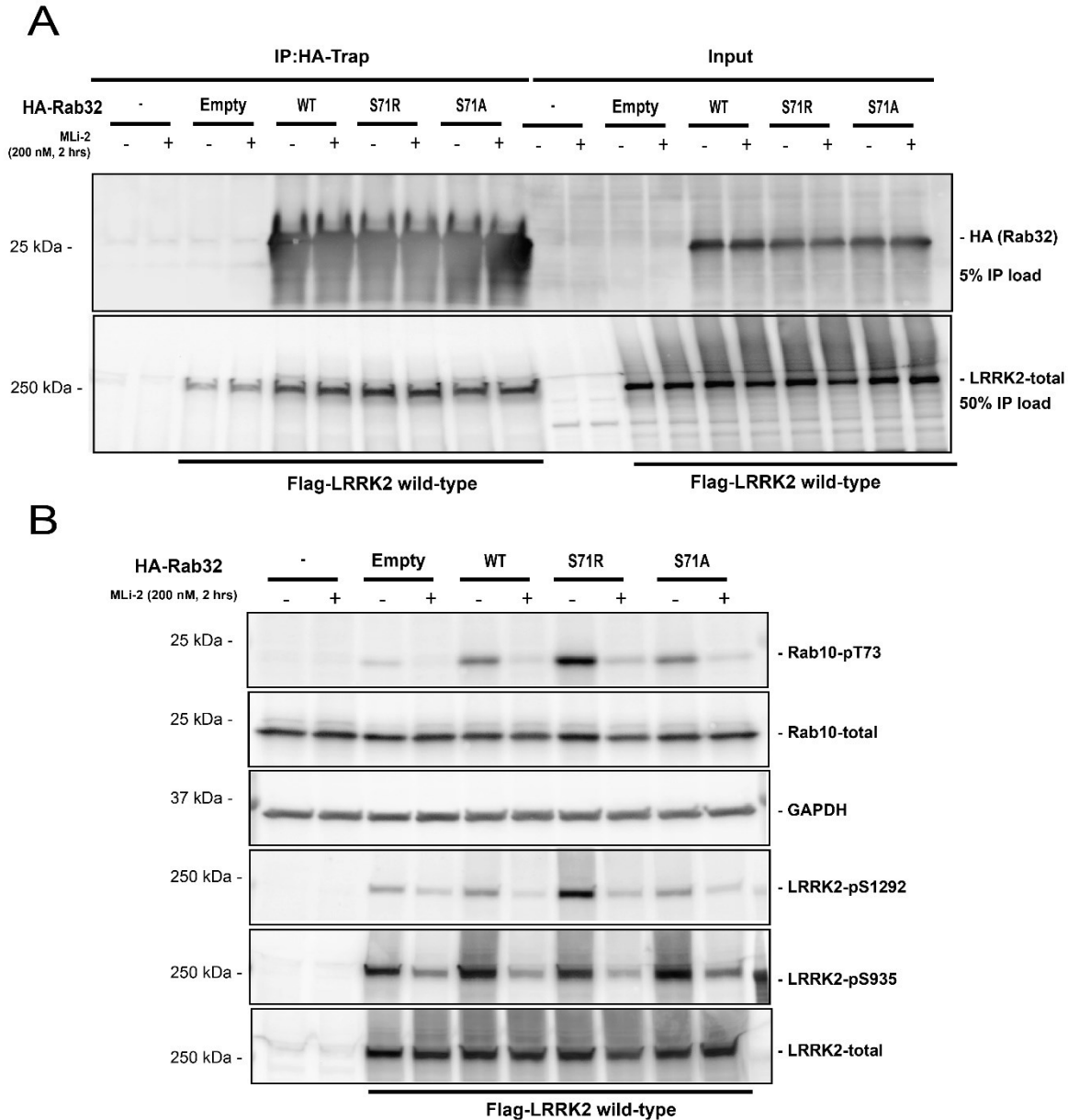
Supplementary figure 6. RAB32 co-immunoprecipitation with LRRK2. A) Immunoprecipitation (IP) analysis of lysates from HEK293FT cells transiently co-expressing 3xFLAG-LRRK2 and either HA empty vector, HA-RAB32 WT or mutant (p.S71R or p.S71A) cDNA. IP with HA-Trap was followed with immunoblot analysis with an anti-HA (top panel) or an anti-FLAG antibody (bottom panel) as indicated. Separate gels from the same IP sample were loaded to limit HA-signal saturation. GAPDH is used for loading control. Input denotes whole cell lysate starting material from HEK293FT cells used for immunoprecipitation analysis; +/- indicates cDNA transfections and Mli-2 treatment. B) Western blot analysis of WCL used in (A) to confirm Mli-2 target engagement was monitored by a loss of pS1292 and pS935 phosphorylation for LRRK2 and pT73 Rab10 for Rab10. Mli-2 was applied at 200nM for 120 mins prior to cell lysis.
