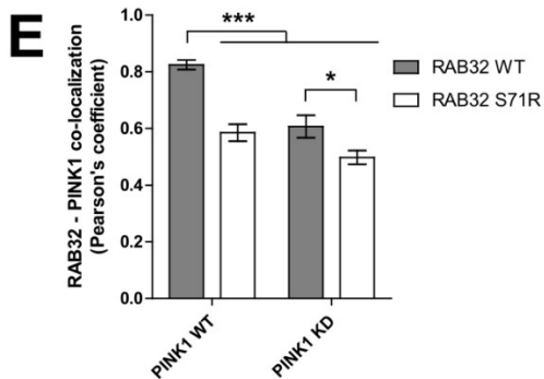
Supplementary figure 7. RAB32 co-localization with PINK1. Confocal images of HEK293 cells co-transfected with mCherry-Parkin and GFP-tagged wild-type RAB32 ( A , B ) or S71R RAB32 ( C , D ) and HA-tagged wild-type PINK1 ( A , C ) or kinase dead PINK1 ( B , D ). Boxes indicate regions shown at higher power below. Scale bars are 10 microns. ( E ) Pearson's correlation coefficient to quantify the co-localization of GFP-RAB32 and HA-PINK1. Bars show mean \pm SEM of 12-15 fields. * indicates P < 0.05 , *** indicates P < 0.0001 according to ANOVA followed by Tukey's multiple comparisons test.
