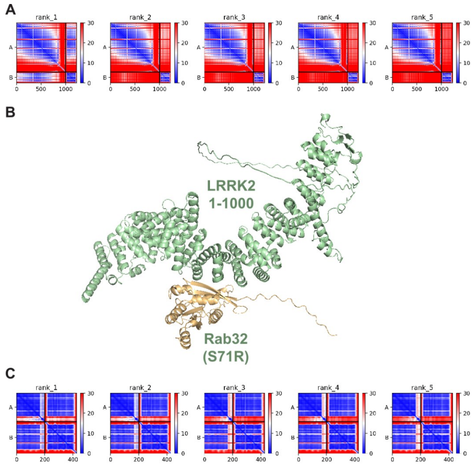
Supplementary figure 5. A) PAE plots of 5 models for the LRRK2(1-1000)/Rab32 prediction. B) Structure overview of the top model for the LRRK2(1-1000)/Rab32 prediction. C) PAE plots of 5 models for the LRRK2(350-550)/Rab32 prediction.
