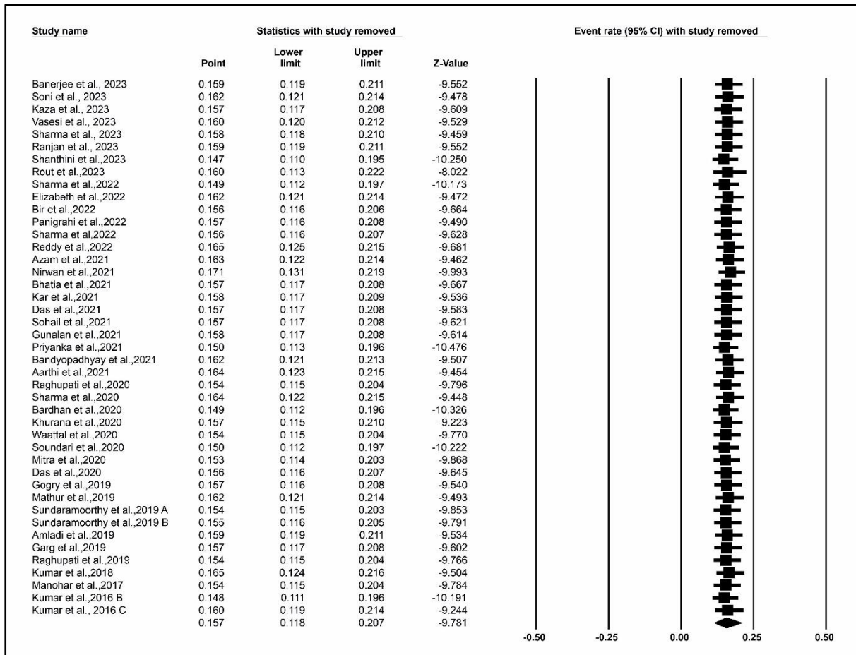
Supplementary Figure 3. Sensitivity plot demonstrating the incidence of polymyxin-resistant bacteria in India.
