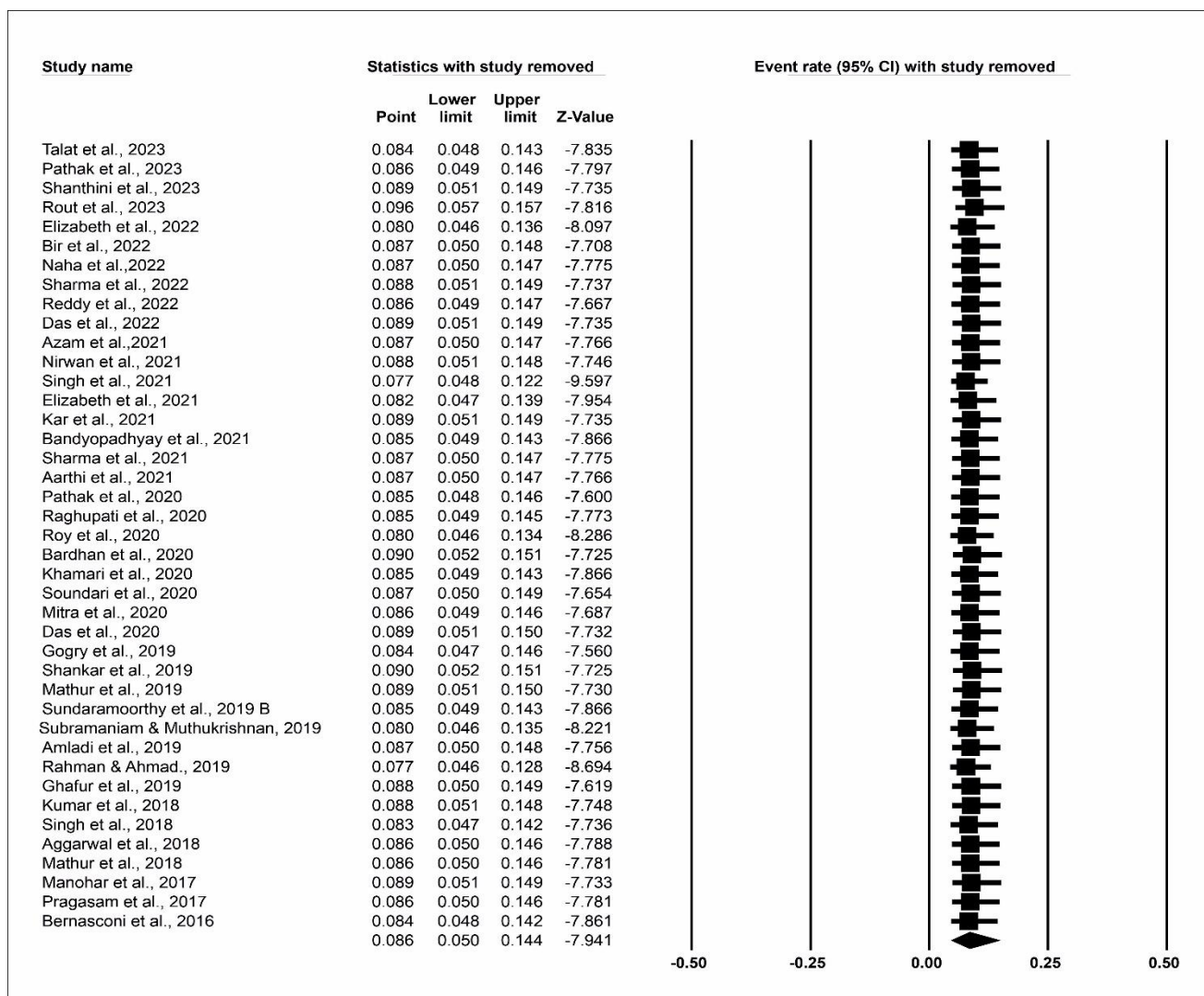
Supplementary Figure 4. Sensitivity plot demonstrating the contribution of the mcr gene in the development of polymyxin resistance in India.
