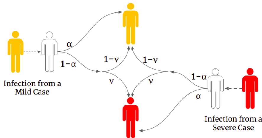
Fig. 3. Dependence of symptom severity on \alpha and \nu (in the absence of interventions). White shaded individuals correspond to those susceptible to infection, yellow shaded individuals correspond to infectious cases with mild severity and red shaded individuals correspond to infectious cases with severe symptoms. The values on the arrows show the corresponding probability. An infected individual has probability \alpha of copying the symptom severity of their infector and a probability 1 - \alpha of reverting to the baseline probability of having severe disease, i.e. they develop severe disease with probability \nu .
