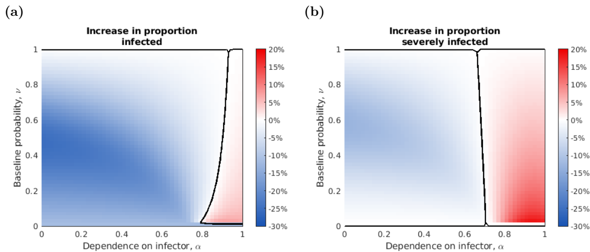
Fig. 4. Investigating the effect of \alpha and \nu on the number of total cases and severe cases prevented by additionally quarantining mild cases. (a) The difference between the overall number of cases when quarantining 50% of severe cases only and the overall number of cases when quarantining 50% of all cases (severe and mild). (b) The difference between the number of severe cases when quarantining 50% of severe cases only and the number of severe cases when quarantining 50% of all cases (severe and mild). Shading denotes the cases prevented (as a percentage of the population): blue denotes values where quarantining mild cases decreased the number of cases; red denotes values where quarantining mild cases increased the number of cases. Black solid lines represent parameter combinations where no cases were prevented by additionally quarantining mild cases.
