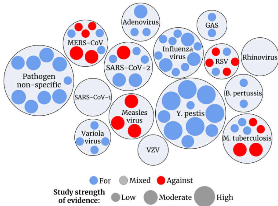
Fig. 2. Infographic depicting the number of relevant studies found for each pathogen for the two symptom propagation mechanisms. The number of relevant studies found for each pathogen relating to (a) dose-severity relationships or (b) route-severity relationships. Colour denotes whether the study was supportive (blue) or against (red) the hypothesis, with mixed studies (grey) containing findings that were both for and against. Bubble size denotes our classification of strength of evidence: high - a study directly investigating symptom propagation with significant findings; moderate - a study strongly related to part of the mechanism with significant findings; low - a study with either non-significant findings, or that is more weakly related to part of the mechanism. All studies are listed in the summary tables with their corresponding strength of evidence ratings (see Supplementary Material File S2).
