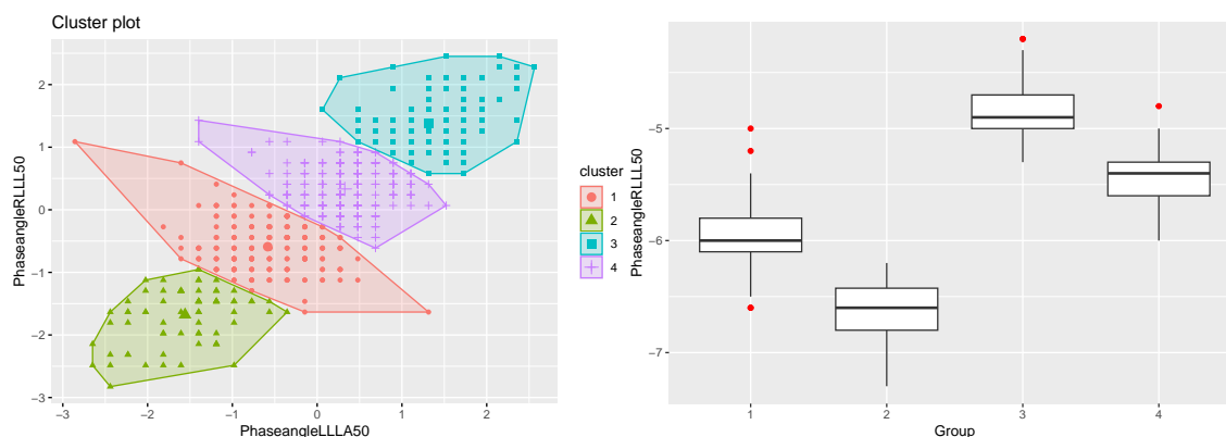
Figure 1: Plots of the four resulting clusters .
