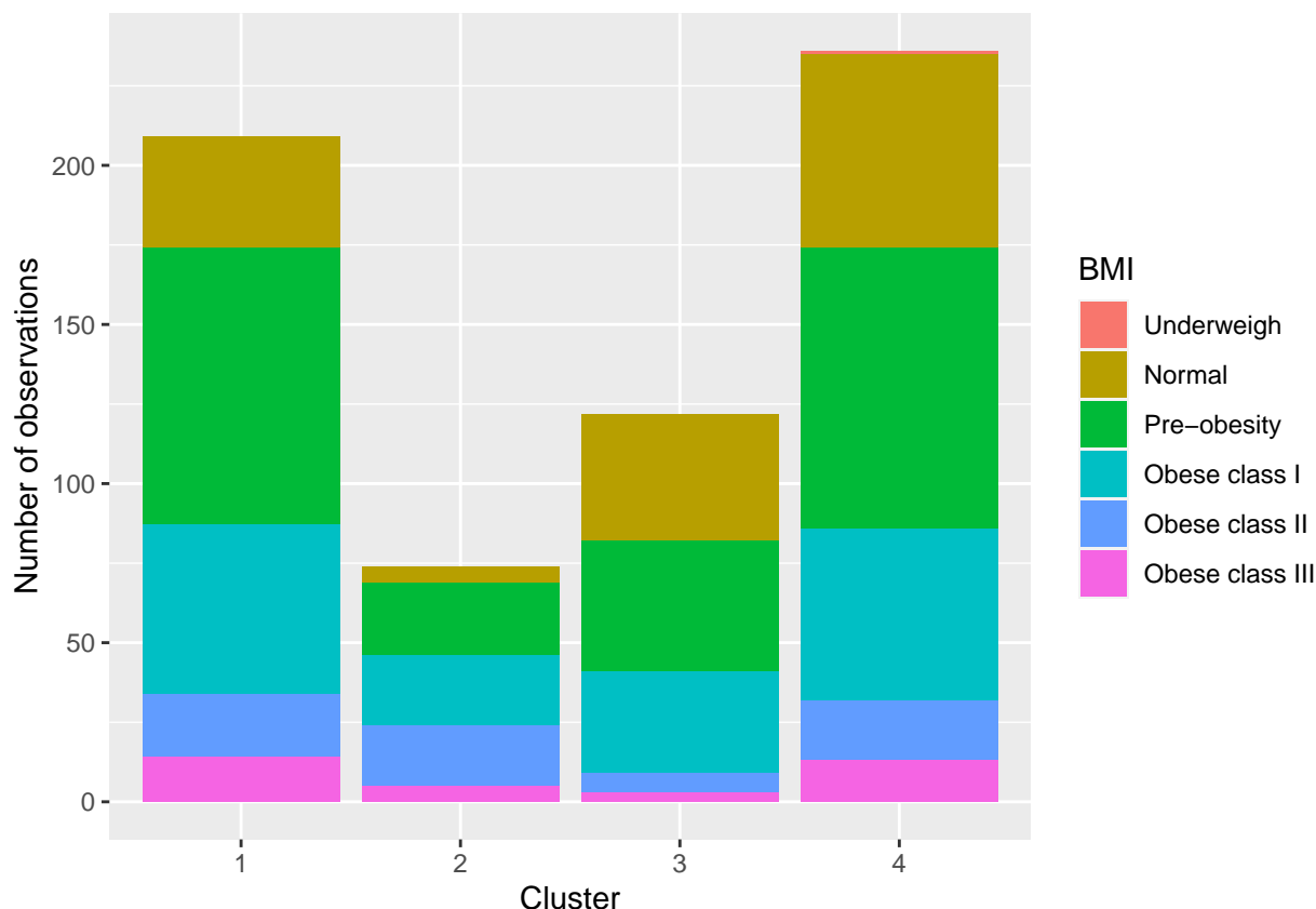
Figure 3: Cluster chart according to the BMI classification reflected in Table 7.
