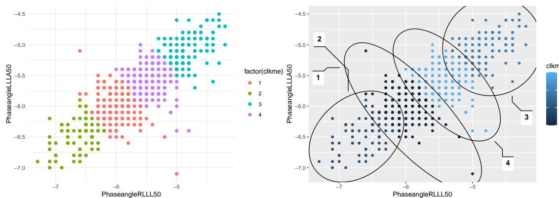
Figure 2: Different representations of the four clusters .
