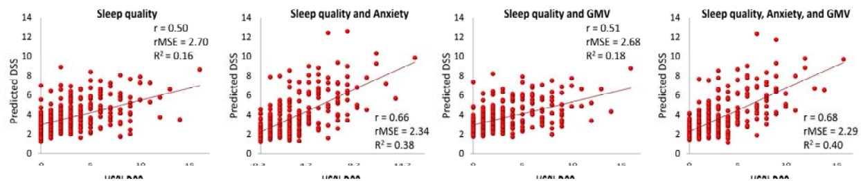
Figure 3. Out-of-cohort validation of ML results in two independent datasets. A) prediction of DSS in HCP-Aging dataset based on sleep quality, a combination of sleep quality and anxiety, a combination of sleep quality and GMV, a combination of sleep quality and anxiety, and GMV; B) prediction of DSS in eNKI dataset based on sleep quality, a combination of sleep quality and anxiety, a combination of sleep quality and GMV, a combination of sleep quality and anxiety, and GMV (GMV: gray matter volume, DSS: depressive symptoms severity after excluding two sleep-related items, r : correlation coefficient between real and predicted DSS, rMSE : root mean squared error, R^2 : determination coefficient)
