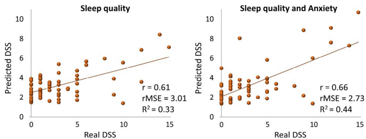
Figure 4. Prediction of future DSS based on sleep quality and anxiety. There were 66 participants in the longitudinal sample of the eNKI dataset (DSS: depressive symptoms severity after excluding two sleep-related items, r : correlation coefficient between real and predicted DSS, rMSE : root mean squared error, R^2 : determination coefficient)
