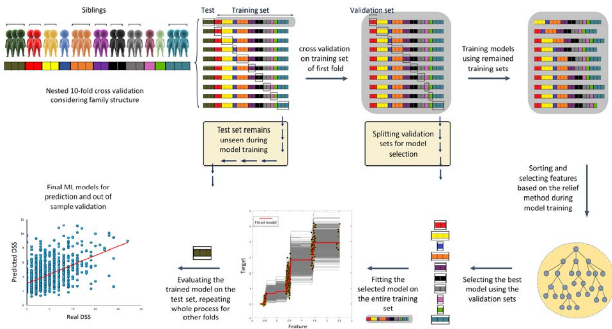
Figure 1. ML pipeline for prediction of DSS (depressive symptoms severity) considering family structure. First of all, 10-fold cross-validation was performed so that siblings were not separated in training/test sets. After putting aside the test set (of the first fold from now), we performed a 10-fold cross-validation on the training set (of the first fold) considering family structure. In this stage, we split validation sets and trained models on the remaining training sets. On each fold, we trained models and optimized hyper-parameters ten times with ten different feature numbers. Hence, we had ten folds and ten models for each fold and the algorithm had to select the model with the best performance and minimum error across all folds. Subsequently, the selected model was fitted on the entire training set and then evaluated on the test set. This process repeated for all other nine folds (Note: all units in the figure are arbitrary, DSS: depressive symptoms severity after excluding two sleep-related items).
