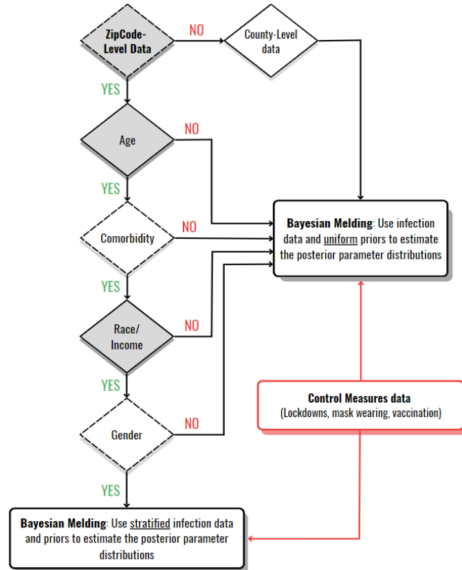
Figure S3: The complexity of the simulator increases as data for age-, comorbidity-, race- and gender-based transmission factors become available at the zip-code or county level.
