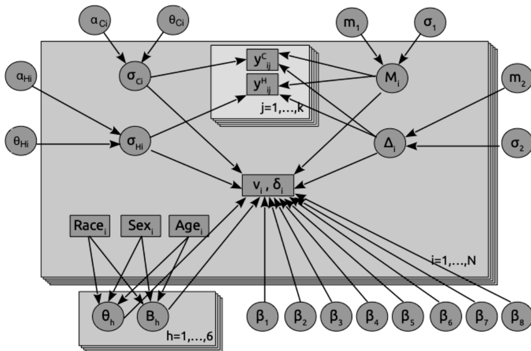
Figure 7: An illustration of the DAG of the mean blood pressure-based model presented in this article.
