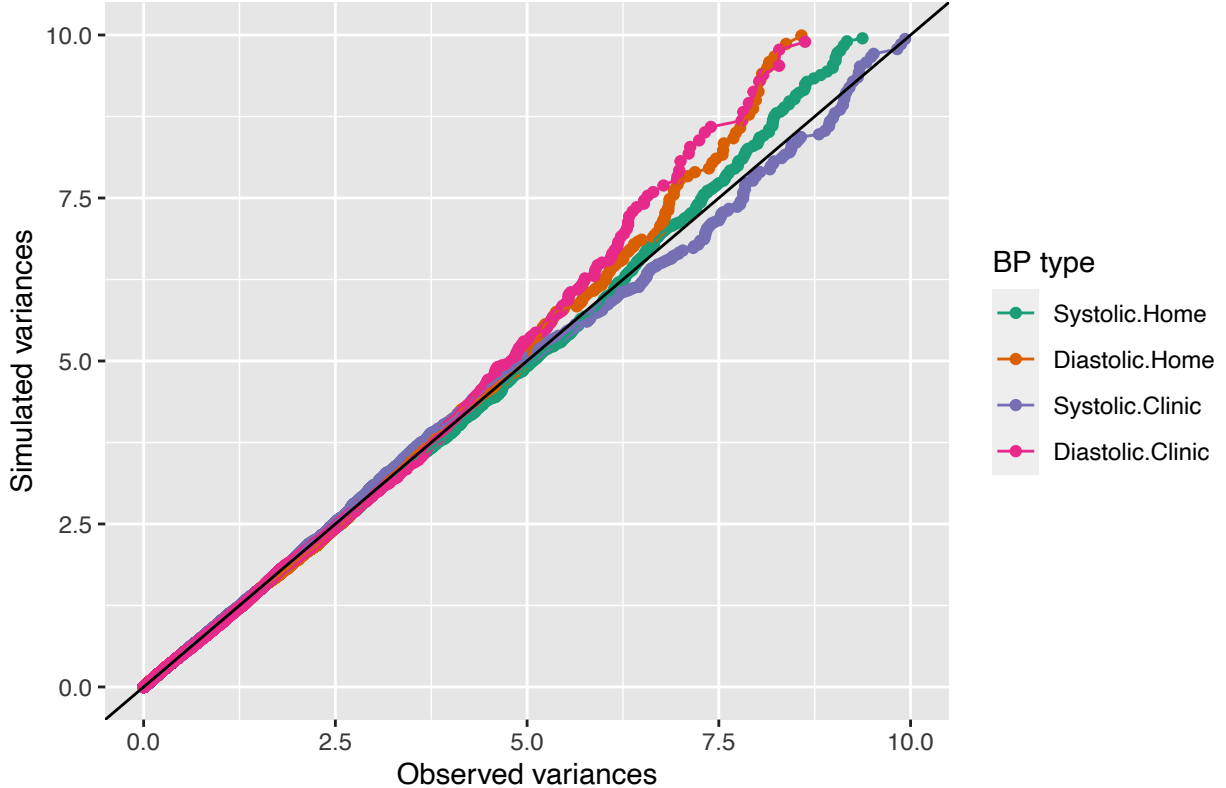
Figure 10: Q-Q plots of the variances of the observed data with imputed fractional parts (x-axis) against the variances of the simulated data (y-axis).
