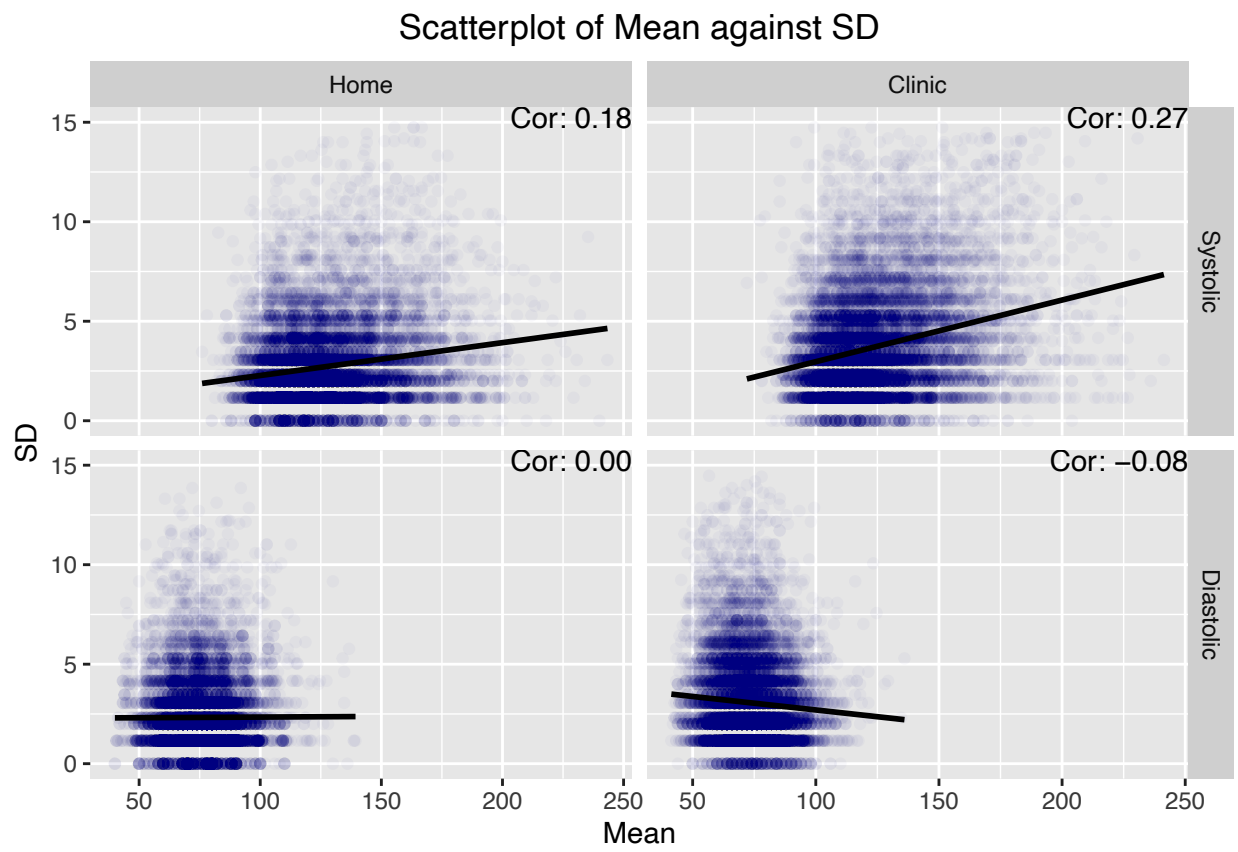
Figure 2: Scatterplot of individual mean BP against individual SD of BP
