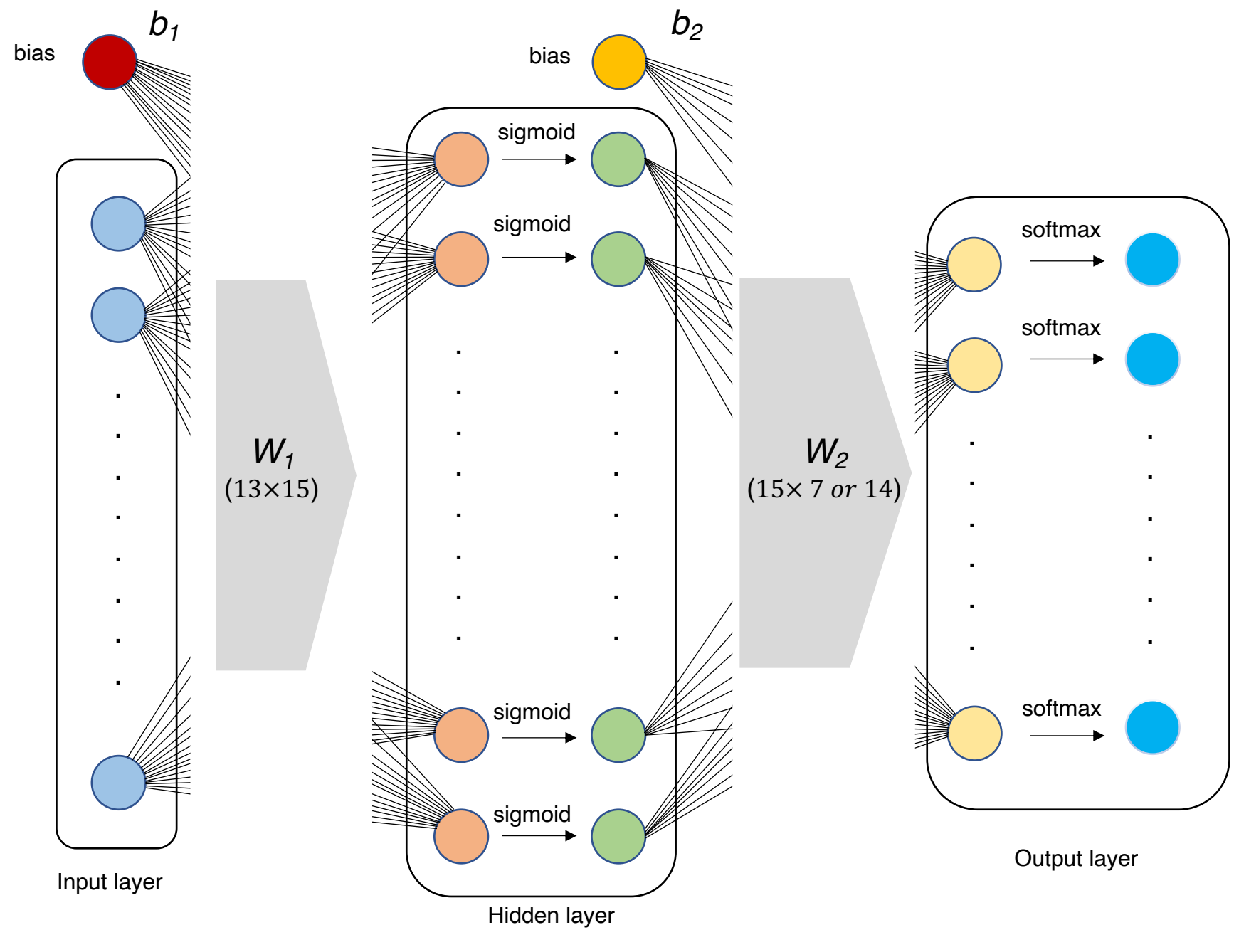
Figure S2. The architecture of the predictive model in this study.
