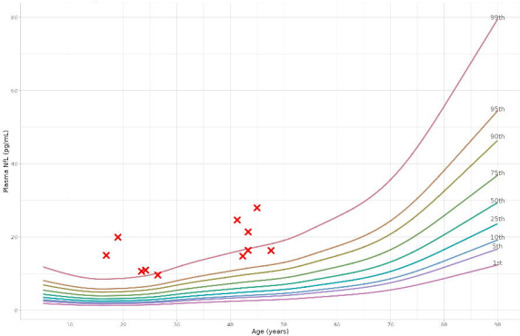
Centile curves using BCT
