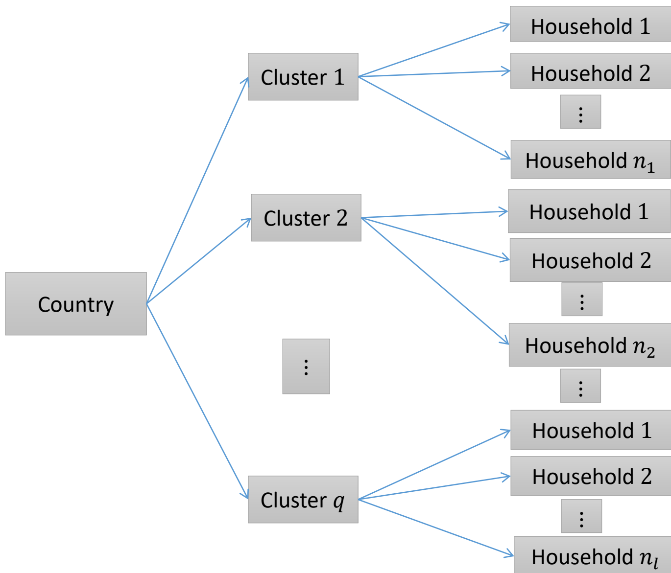
Figure 1. Survey structure
