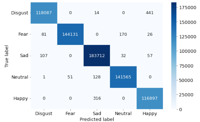
Fig. 5. Confusion matrix
