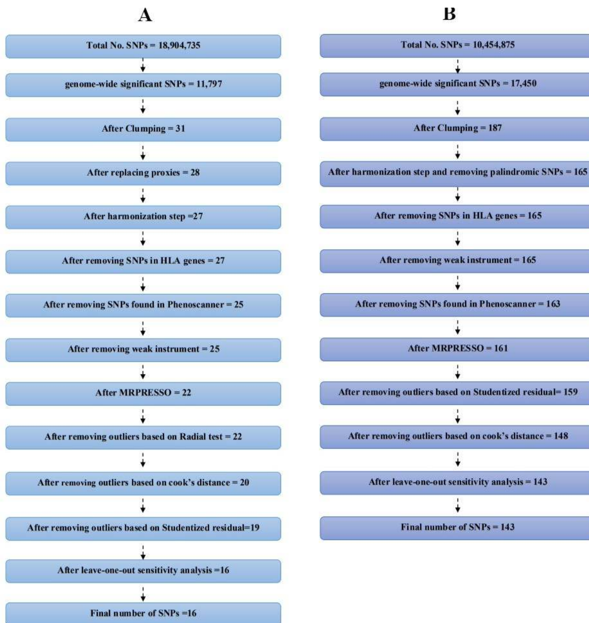
Figure 2: Selecting an appropriate instrumental variable (IV) in Mendelian randomization is a crucial step because the validity of your causal inference depends on it. Here are the key steps involved in the selection of an IV in Mendelian randomization. Genome-Wide Significant SNP: In this step, researchers identify a genetic variant (SNP) that is genome-wide significant in genome-wide association studies (GWAS) for the exposure of interest. Genome-wide significance means that the SNP is highly associated with exposure. Clumping: Clumping involves selecting a subset of SNPs in linkage disequilibrium with the primary SNP. Replacing Proxies: Sometimes, the initial genome-wide significant SNP is not qualified as an instrumental variable due to issues like pleiotropy or linkage disequilibrium with other SNPs. In such cases, the primary SNP is replaced with a proxy SNP that has a similar effect on the exposure but fewer issues. Harmonization Step: Data harmonization is the process of standardizing genetic data from different sources or studies to ensure compatibility. This step is crucial when combining data from multiple datasets. Removing HLA Gene: The HLA (Human Leukocyte Antigen) gene region is known for its extensive genetic diversity and complex associations with various traits. In MR analysis, it's common to exclude SNPs in the HLA region to minimize potential confounding or pleiotropic effects. Check Phenoscanner: Phenoscanner is a tool used to explore genetic
