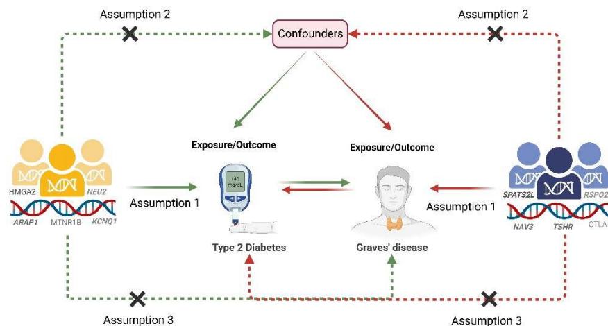
Figure 1: Mendelian randomization is a statistical technique used in epidemiology and genetics to assess causal relationships between an exposure (e.g., a risk factor) and an outcome (e.g., a disease). It relies on genetic variants that are randomly inherited at conception to mimic the randomization process of a controlled experiment, helping researchers infer causal relationships. Figure 1 shows the framework of two sample bidirectional Mendelian randomization analysis is based on several key assumptions. 1: The genetic variations are strongly associated with exposure; 2: The genetic variations are not associated with either known or unknown confounders; 3: SNPs should influence risk of the outcome through the exposure, not through other pathways. The green line represented the Mendelian randomization analysis of the association of GD with T2D. The red line represented the Mendelian randomization analysis of the association of T2D with GD.
