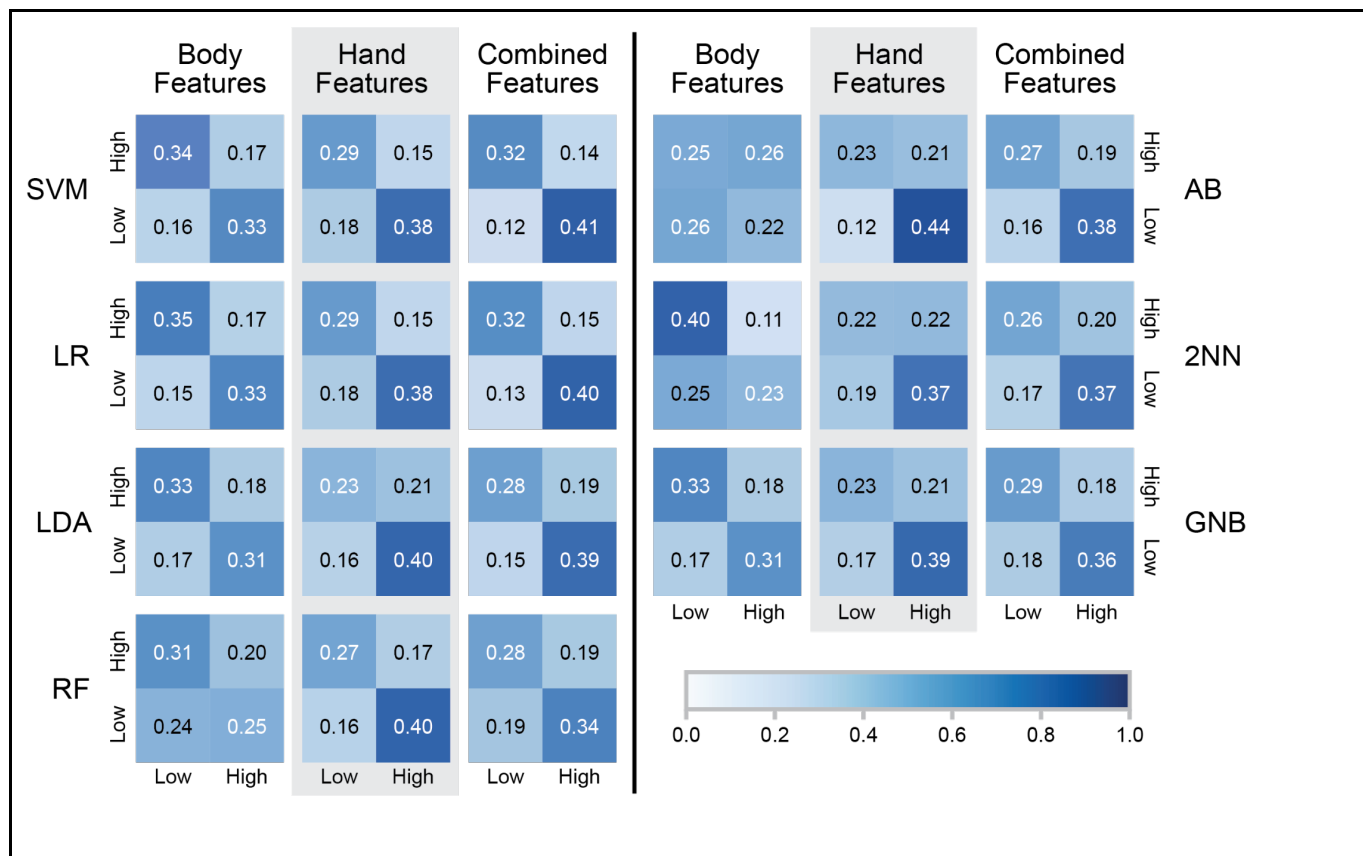
Supplemental Figure 3: Average confusion matrices of selected classifiers. LDA = linear discriminant analysis; LR = logistic regression; SVM = support vector machine; RF = random forest; AB = adaptive-boosted trees. Compared to classifiers trained with gait features, classifiers trained with finger-tapping features misclassified the low motor impairment class more. Classifiers trained with both gait and finger-tapping features had more confidence and accuracy when predicting the motor impairment labels.
