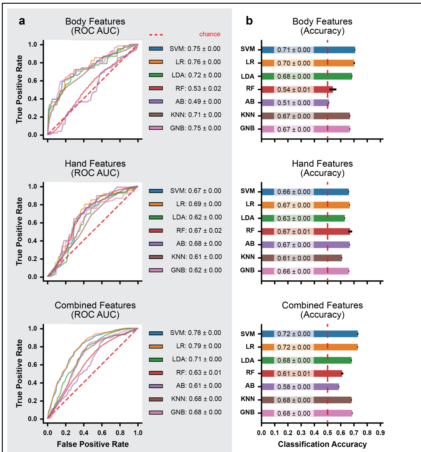
Figure 2: Classification performances of seven selected ML classification models. SVM = support vector machine; LR = logistic regression; LDA = linear discriminant analysis; RF = random forest; AB = adaptive-boosted trees; KNN = K-nearest neighbors; GNB = Gaussian naive Bayes; ROC AUC = area under receiver operating characteristics curve. a. Here we show the average ROC curves of the trained ML models during 16-times repeated leave-on-subject-out cross-validation (CV). The corresponding AUC scores are reported in the right margins as mean ± standard deviation. Overall, integrating body and hand features led to improved performances in the most models. b. Here we
