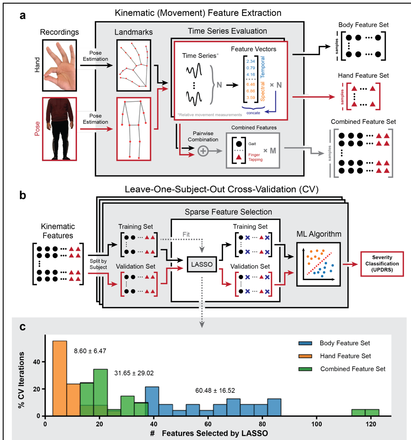
Figure 1: Schematic overview of automatic feature extraction from video recordings for classification of Parkinson's disease motor symptom severity. a. From recordings of participants performing prescribed motor assessment tasks, we extracted movement (kinematic) time series at key landmarks using the pose estimation library MediaPipe. Relative movement measurements were computed based on the extracted signals, from which various temporal and spectral metrics were computed as features. Pairwise combinations of samples from the same patient under the same medication state were performed on the body and hand feature sets to form the bi-modality
