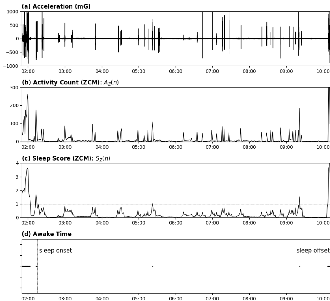
Figures 4. Acceleration Signal to Sleep/Wake Detection (ZCM).
