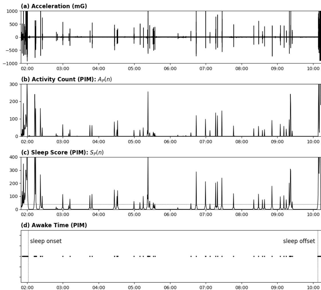
Figures 3. Acceleration Signal to Sleep/Wake Detection (PIM).
