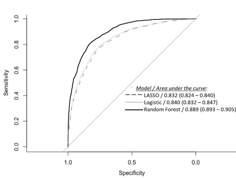
Figure 2: Receiver operating characteristic curves (a) and calibration plot (b; Random Forest model only) for prediction models in test dataset
