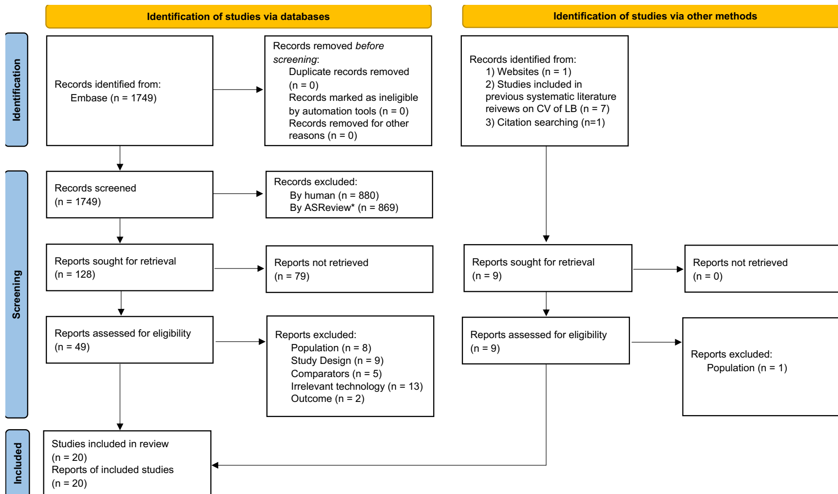
Figure 1. The PRISMA flowchart of included studies
