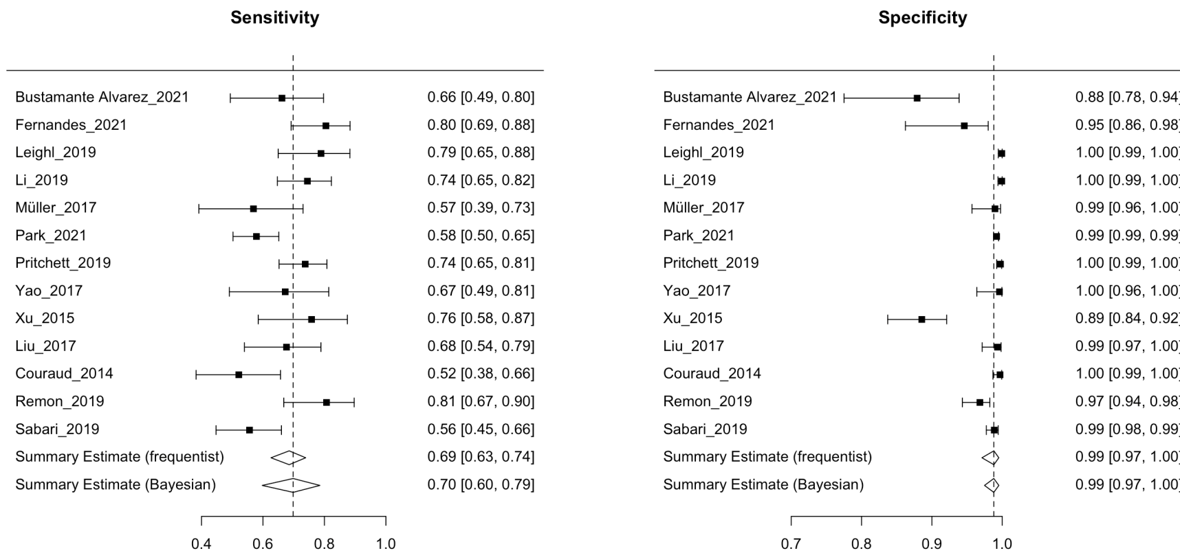
Figure 2. Forest plot of sensitivity and specificity of ctDNA testing for multi-gene detection from bivariate random effects meta-analyses (n=13)
