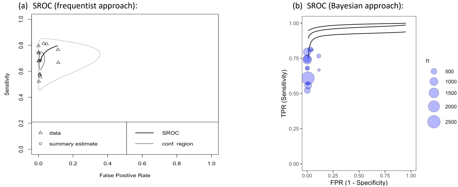
Figure 3. Summary receiver operating characteristics (SROC) plots based on frequentist and Bayesian bivariate random-effects meta-analyses (n=13)
