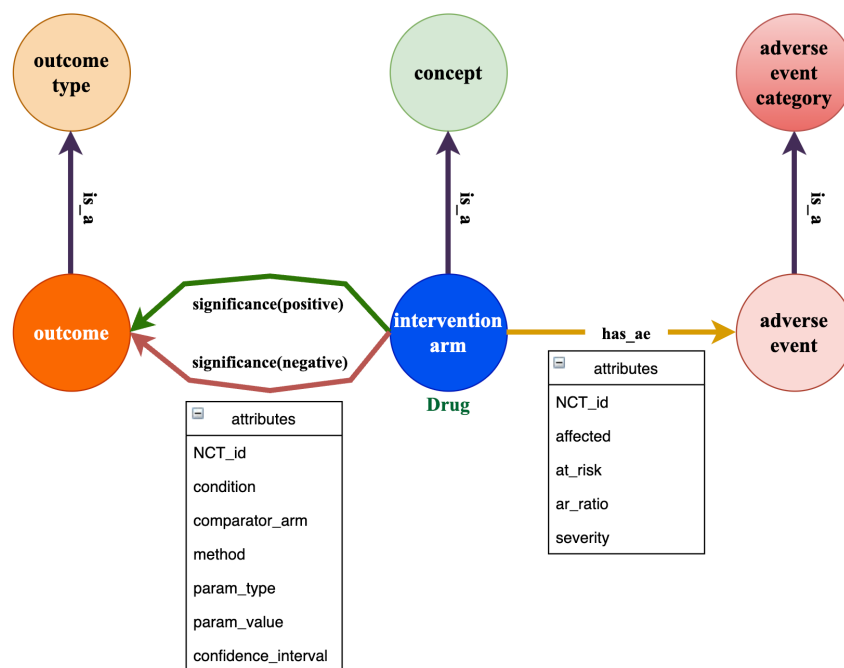
Figure 3. An overview of the schema of arm-level efficacy and safety knowledge graph
