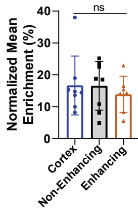
B Ribose-5-P (human)
