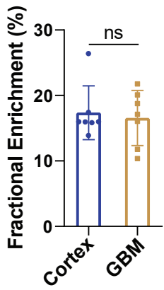
A Ribose-5-P (mouse)
