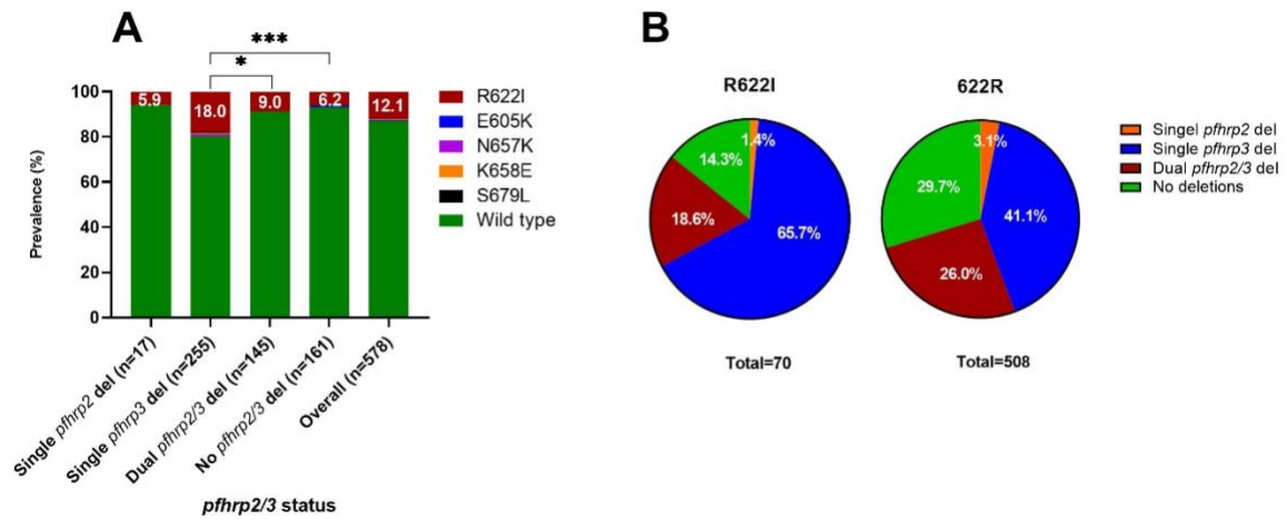
Supplementary Figure 1. Prevalence K13 mutations in samples with different pfhrp2/3 status (A) and proportion of pfhrp2/3 -deleted parasites among K13 R622I mutant and 622R wild type (B).
