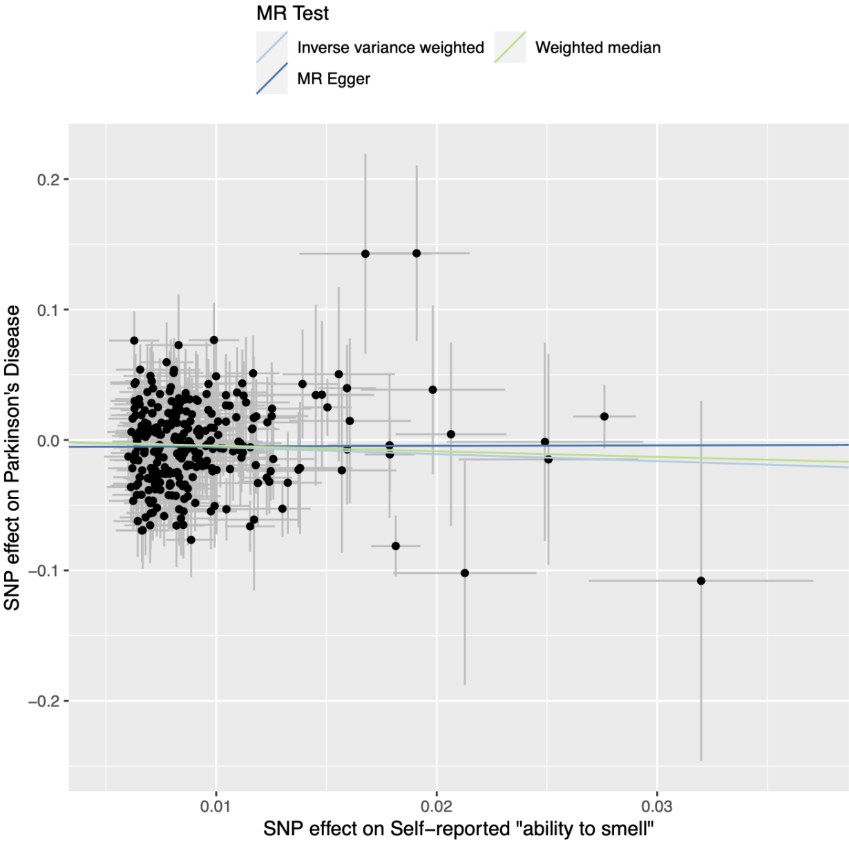
Supplementary Figure 5 - Scatter plot of outlier-removed reverse-causation MR results
