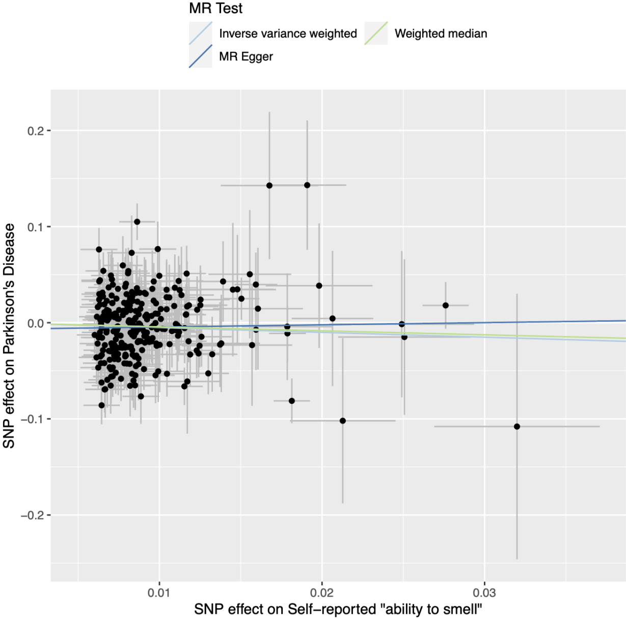
Supplementary Figure 4 - Scatter plot of reverse-causation MR results
