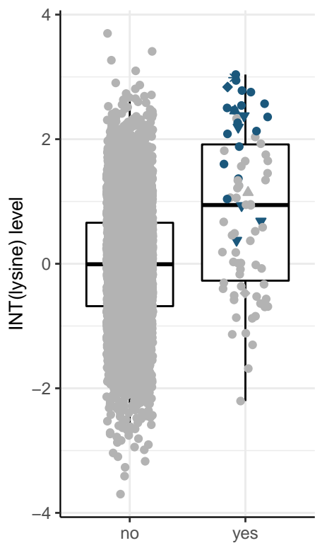
putative functional alleles at SLC7A9 (HI_mis)
