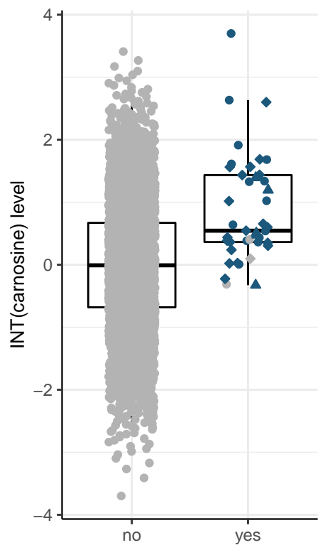
putative functional alleles at CNDP1 (LoF_mis)
