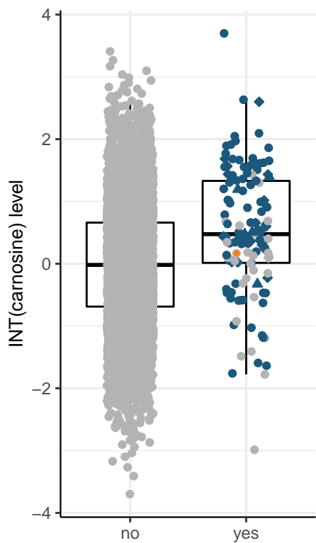
putative functional alleles at CNDP1 (HI_mis)
