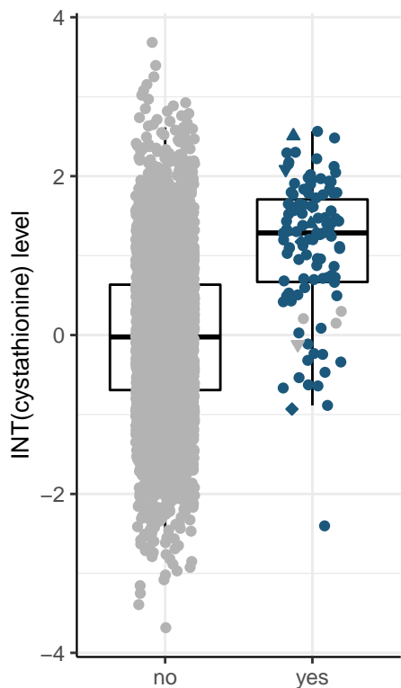
putative functional alleles at CTH (HI_mis)
