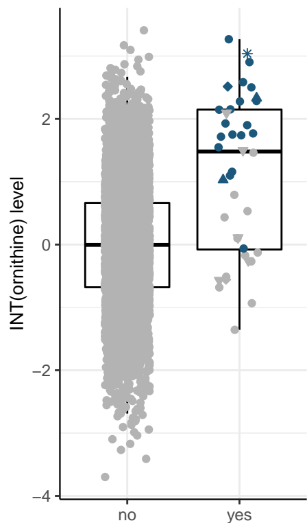
putative functional alleles at SLC7A9 (LoF_mis)
