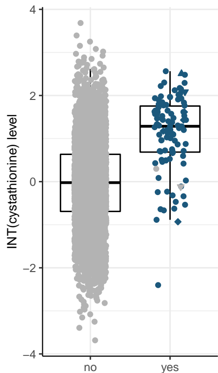
putative functional alleles at CTH (LoF_mis)
