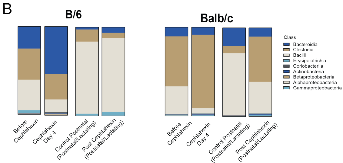
Supplementary Figure 3: A) Stacked bar plots of relative abundance of families in B/6 and BALB/c dam stool. B) Stacked bar plots of pooled relative abundance of classes in B/6 and BALB/c dam stool.
