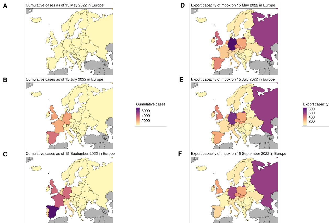
Figure S6. Cumulative number of reported mpx cases and the estimated export capacity in Europe
