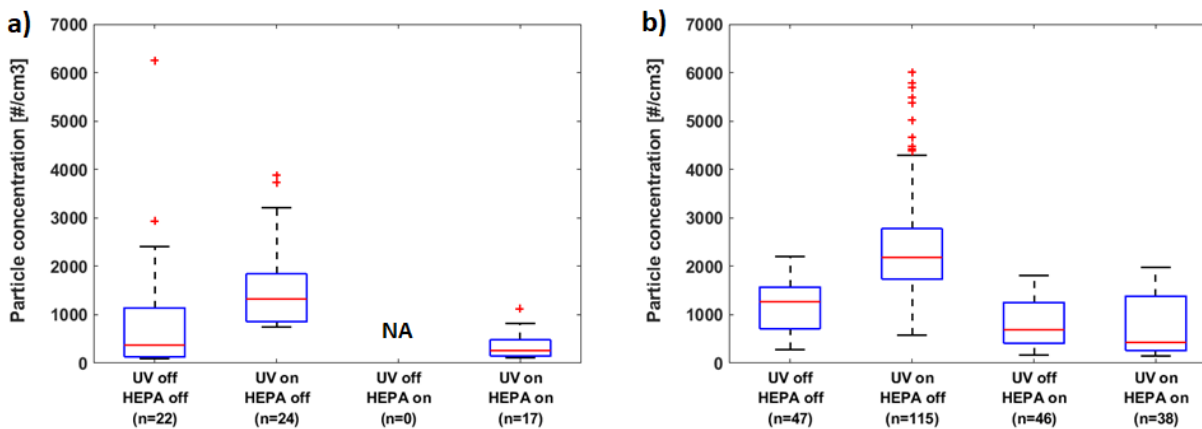
373 Figure 7. Ultra-fine particle concentrations (17.5 to 289 nm) with and without use of 222 nm far-UVC 374 lamps and HEPA filters a) in the sealed unfurnished room (no data from HEPA on UV off) and b) in the 375 standard room. Boxplots show medians (redline inside the boxes), 25th and 75th percentiles (top and 376 bottom of the boxes), most extreme data not considered outliers (whiskers) and outliers (red crosses) of 377 1-hr data. n represents the number of 1-hr data points included in each boxplot. HEPA filter units 378 delivered 232 L/s (9.1 ACH) in the sealed room and 116 L/s (7.1 ACH) in the standard room. Simultaneous 379 background measurements to account for indoor and outdoor sources were not collected.
