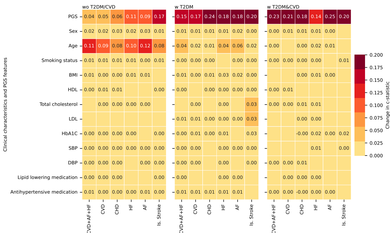
Figure 19: The contribution of each clinical feature to the prediction of cardiovascular disease.
