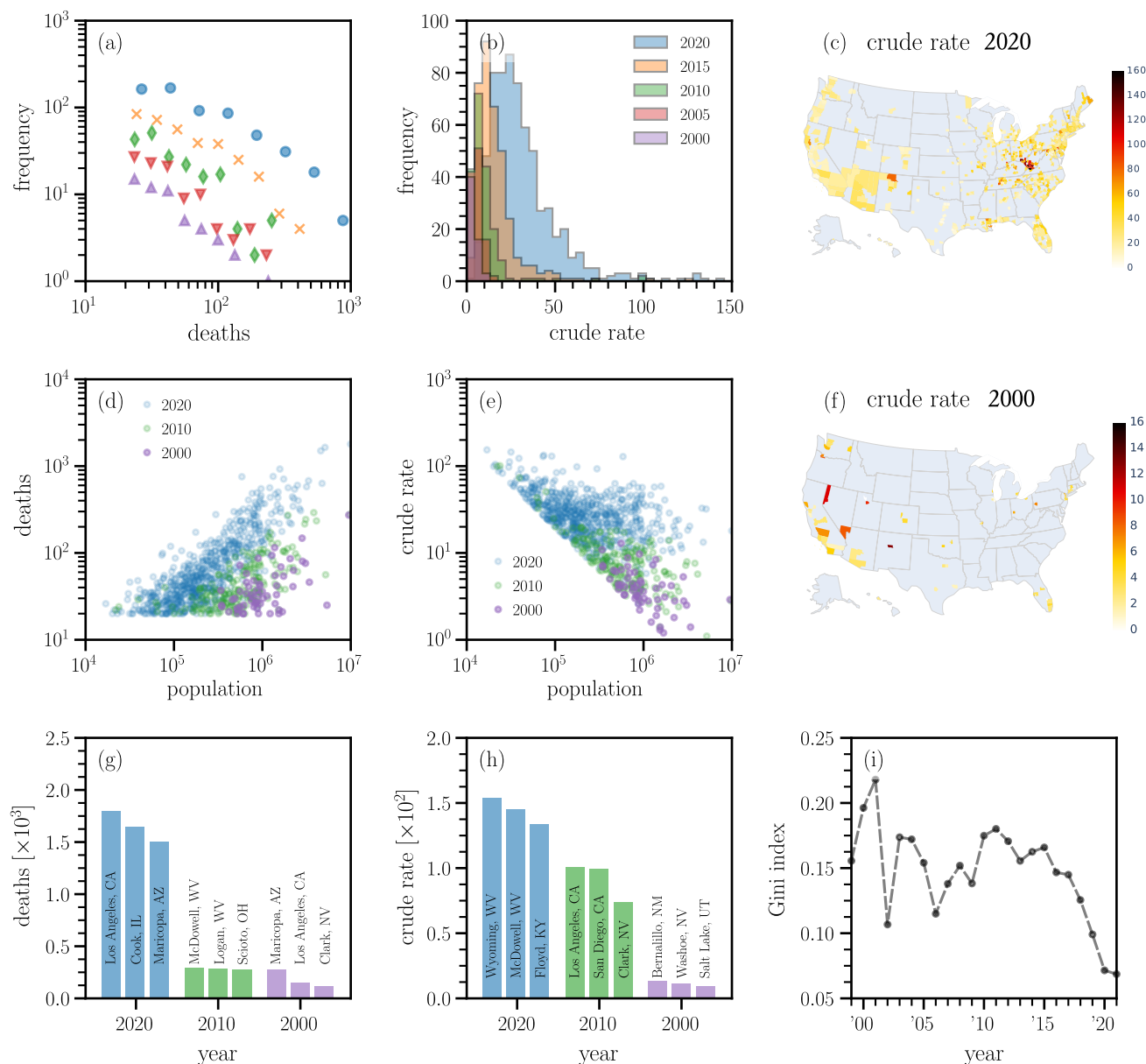
FIG. 3. Drug-overdose fatalities in the United States at the county level. (a) Histogram of county-stratified drug-overdose fatalities for different years (blue disks: 2020, orange crosses: 2015, green diamonds: 2010, red inverted triangles: 2005, purple triangles: 2000). (b) Histogram of county-stratified crude rate data for different years. (d) County-stratified drug-overdose fatalities as a function of the corresponding county populations. (e) County-stratified crude rates as a function of the corresponding county populations. (c,f) Crude rates across different counties in 2020 and 2000. The scales of the two color bars differ by a factor of 10. In the gray regions, either no data or a statistically not significant number of cases were reported. In all panels, we did not include data for which at least one database entry ( e.g. , fatalities and crude rate) was marked unreliable. The minimum number of deaths in the remaining data is 20. Hence, the crude rate data in (e) lies above of the minimum crude rate given by 2 \times 10^6 / \text{Population} . (g) The three counties with the largest overdose death tolls in 2020, 2010, and 2000. (h) The three counties with the largest overdose crude rates in 2020, 2010, and 2000. (i) The Gini index across different years. A Gini index of 0 means that the crude rate is the same across all counties. If all overdose fatalities were concentrated in one out of N_c counties, the Gini index would be 1 - 1/N_c . The number of counties with statistically significant fatality counts (greater than 10 deaths in a given year) and crude rates are N_c = 61 in 1999 and N_c = 742 in 2021.
