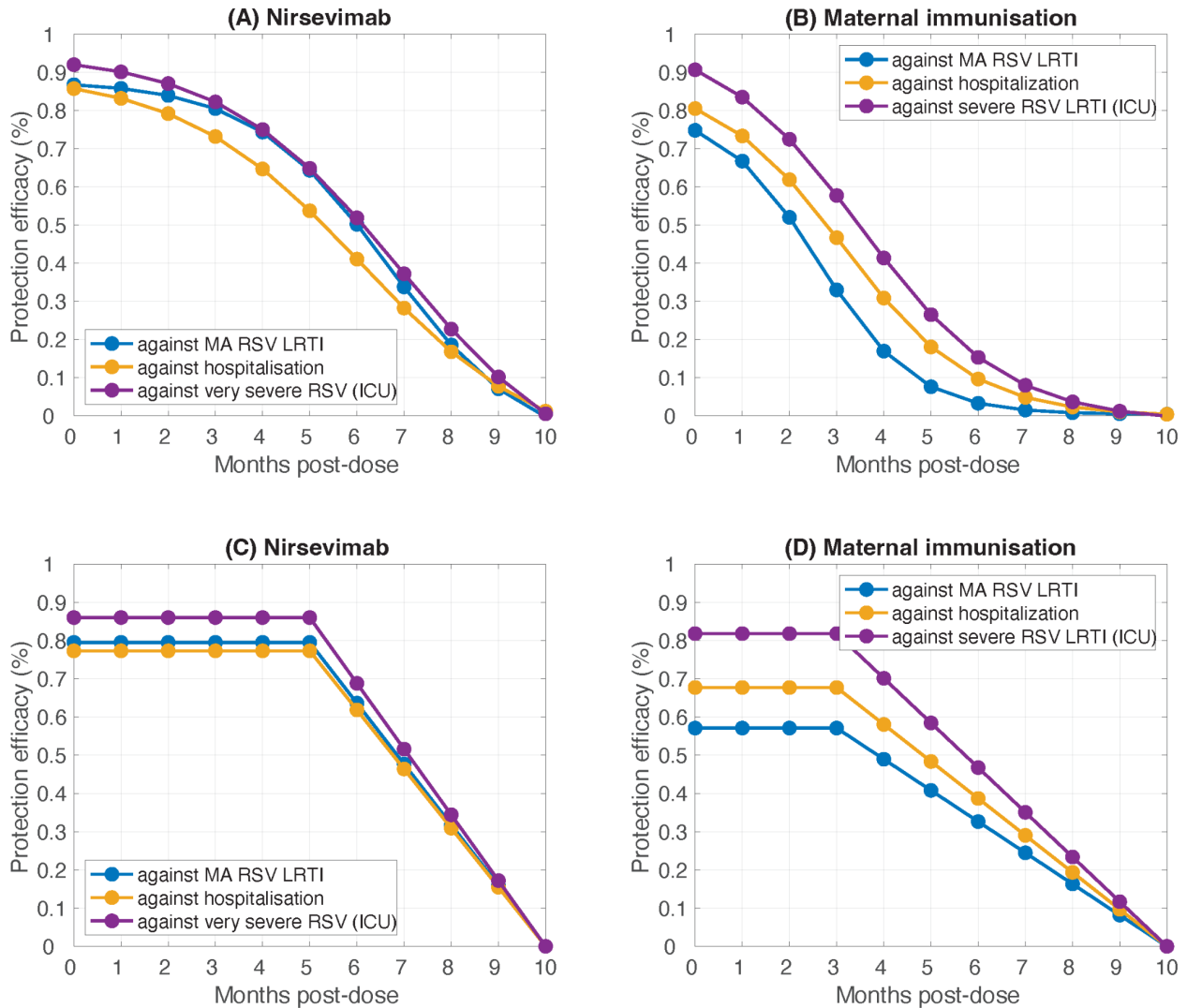
Figure A4. Vaccine efficacy profiles. Panel (A) and (B) correspond to sigmoidal decay of protection for each outcome after a single dose of nirsevimab and RSVpreF, respectively. Panel (C) and (D) correspond to constant protection efficacy followed by a linear decline to zero after a single dose of nirsevimab and RSVpreF, respectively.
