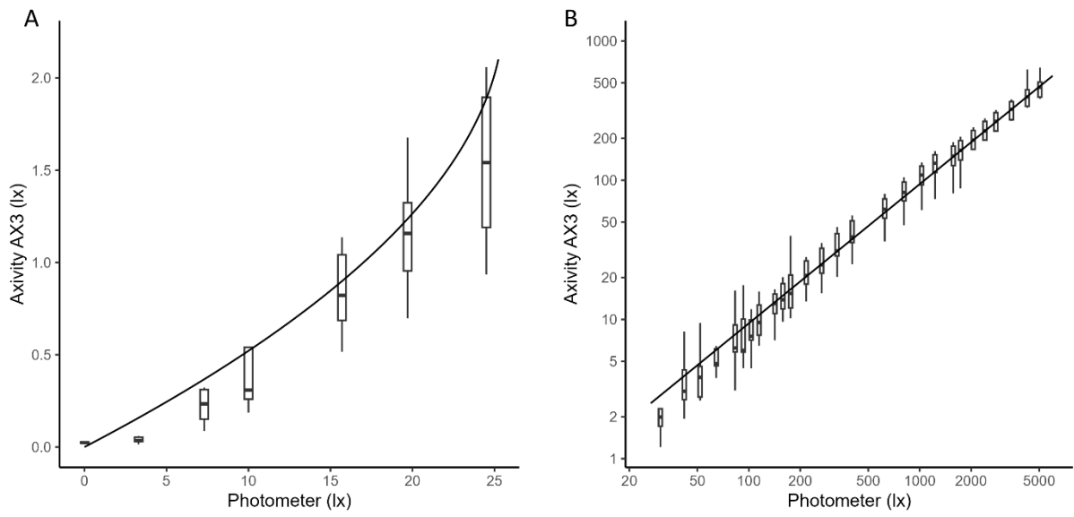
Figure S5. AX3 validation: light intensity for device output vs. reference photometer. Test data were split into (A) 0-25lx photometer range (non-linear device response), and (B) 25-5500lx photometer range (linear device response)
