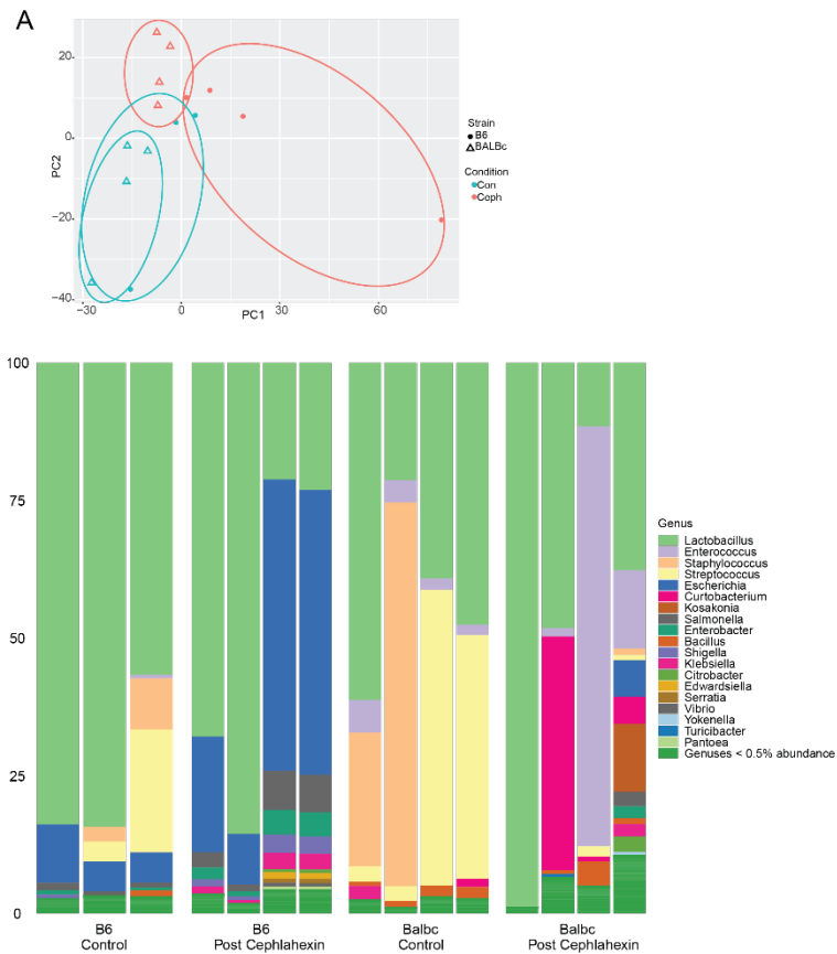
Supplementary Figure 2: A) Principal component analysis of 16S sequencing revealed similar microbiota composition of control pups (blue=control; closed circles=C57BL/6, open triangles = BALB/C), but differing effects of cephalixin (pink=cephalexin). B) Stacked bar plots of relative abundance of genus taxa in B/6 and BALB/c pup stool. N=3 independent litters per group.
