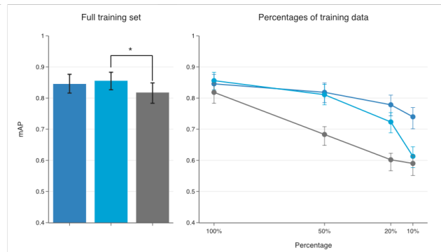
b Mean average precision of lesion anatomical site classification for the full training set and percentages of training data
