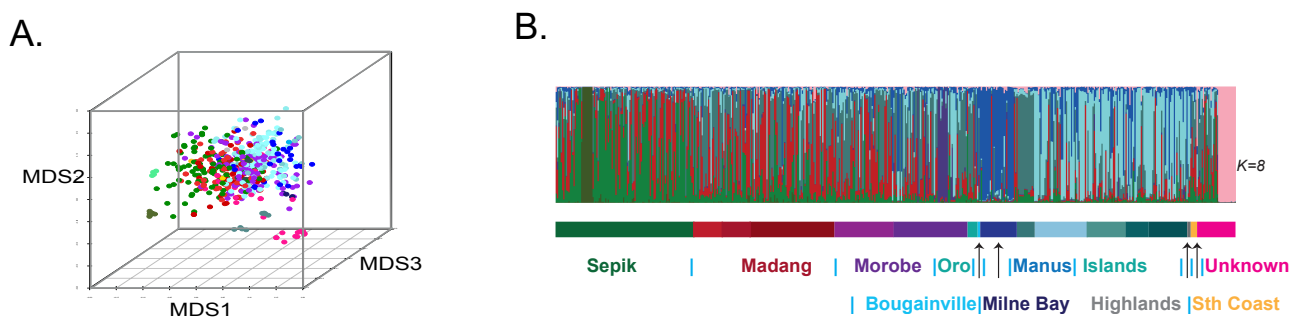
Figure 5. Population structure of P. falciparum in Papua New Guinea. A) MDS analysis of the outbreak samples with all PNG samples. B) Ancestry coefficients (min = 0 max =1) of outbreak samples with all PNG samples using Bayesian cluster analysis. Colours match geographical origins as indicated on the map in Figure 2A. Unknown genotypes (pink) correspond to clinical samples of unknown geographical origin from migrating workers as described in the next section.
