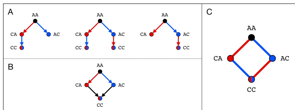
Figure 1. Reticulate events in molecular evolution create topological cycles. (A) and (B) show possible evolutionary histories on the level of individuals in the example of a genome with only two nucleotides. The coloring of the edges corresponds to the acquisition of a specific mutation, while the coloring of the nodes represents individuals carrying this mutation. Convergent evolution (A) or recombination (B) leads to the presence of four alleles for which there is no single consistent phylogeny (four-gamete test). On the genomic level, genetically identical individuals cannot be distinguished and incompatible phylogenies are represented by a topological cycle in the corresponding phylogenetic network (C).
