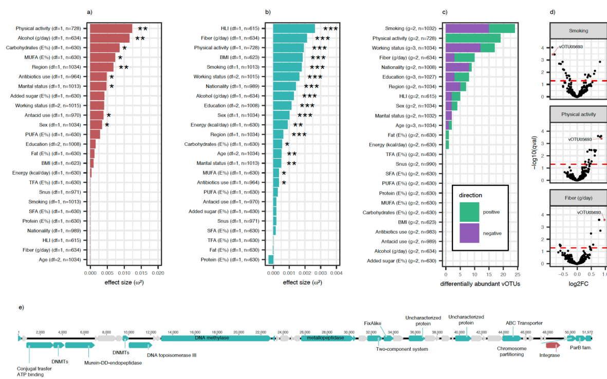
Figure 5: Associations of viral diversity with diet, lifestyle and demographic variables. a) Effect sizes of alpha diversity of vOTU abundance as measured by the inverse Simpson index by ANOVA. b) Effect sizes of associations between vOTU beta diversity (Bray-Curtis index) by PERMANOVA. Effect sizes for alpha and beta diversity are derived using the omega squared measure from ANOVA tests of the association between diversity measures and each variable, with correction for sample sequencing coverage. * p < 0.05 , ** p < 0.01 , *** p < 0.001 . c) Number of significantly differentially abundant vOTUs identified by MaAsLin2, colored by direction of association. For continuous variables, the top and bottom tertiles were compared. d) Volcano plots showing the relationship between effect size (log2 fold change) and significance level (q-value) for vOTUs for physical activity, smoking and fiber intake, from top to bottom. The red dotted line indicates the significance threshold. MUFA: mono-unsaturated fatty acids, PUFA: poly-unsaturated fatty acids, TFA: trans fatty acids, SFA: short-chain fatty acids, BMI: body mass index, HLI: healthy lifestyle index. e) Genomic map representation of CRCbiome_vOTU05693, associated with smoking, physical activity and dietary fiber intake, with predicted genes with annotations in green, without annotations in gray, and integrase gene annotation highlighted in red.
