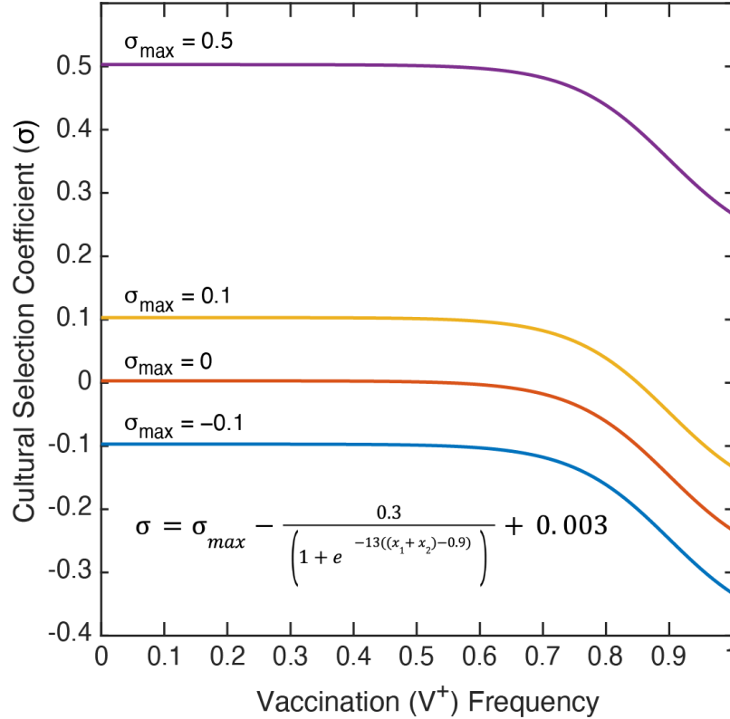
Figure S1: Cultural selection coefficient function. The cultural selection coefficient considers both health and non-health related effects, and the function was constructed by fitting a curve to specified conditions. The selection coefficient ( \sigma ; vertical-axis) is dependent on the frequency of vaccinated individuals ( V^+ ) in the population (horizontal-axis). \sigma_{max} is the maximum cultural selection coefficient associated with being vaccinated. Perceived vaccine benefit is reduced as vaccination coverage increases, since the negative effects of the disease will be less apparent.
