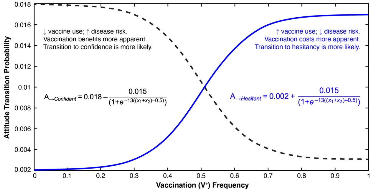
Figure S2: Attitude Transition Probability Function. Attitude transition probability functions were constructed by fitting a curve to specified values. Attitude transition probability (vertical axis) is a function of the vaccination frequency in the population ( V^+ ; horizontal axis). The probability that a vaccine hesitant individual adopts vaccine confidence ( A^- to A^+ transition probability, shown in black) is determined by the function A_{\rightarrow \text{Confident}} , and the probability that a vaccine confident individual adopts vaccine hesitancy ( A^+ to A^- transition probability, shown with a blue dashed line) is determined by the function A_{\rightarrow \text{Hesitant}} .
